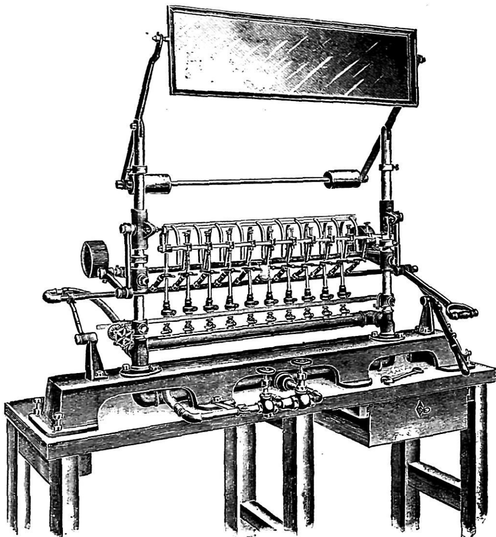
FIG. 17.—Burning Off and Hardening Machine for Inverted Mantles, \frac{1}{4} Actual Size.
