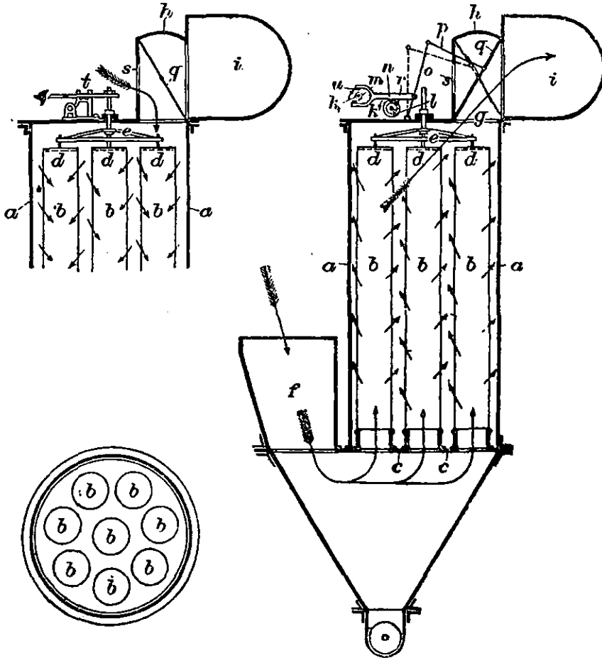
FIG. 29.—The Beth Dust Collector.
