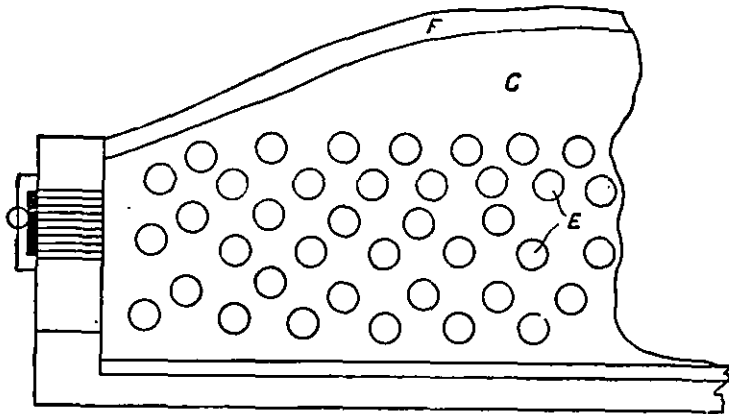
FIG. 4.—Furnace for Graphitising Electrodes.
