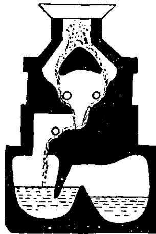
FIG. 4.—Diagrammatic Section of Becker's Electric Furnace.
