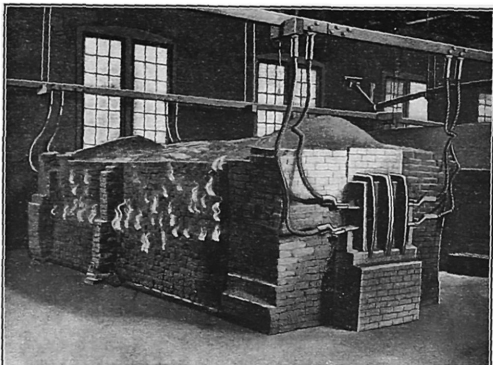
FIG. 2.—Fitz-Gerald's Carborundum Furnace in Action.
