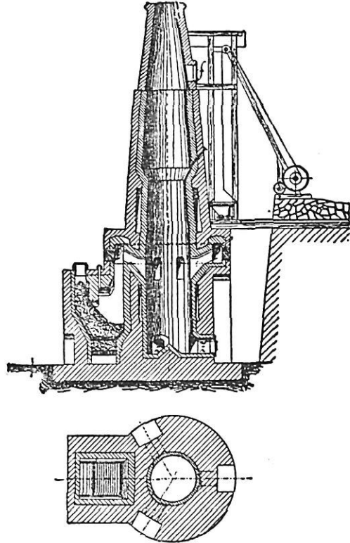
FIG. 4.—Schmatolla's Kiln.
