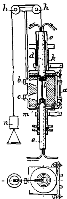
FIG. 12.—Electric Furnace.
