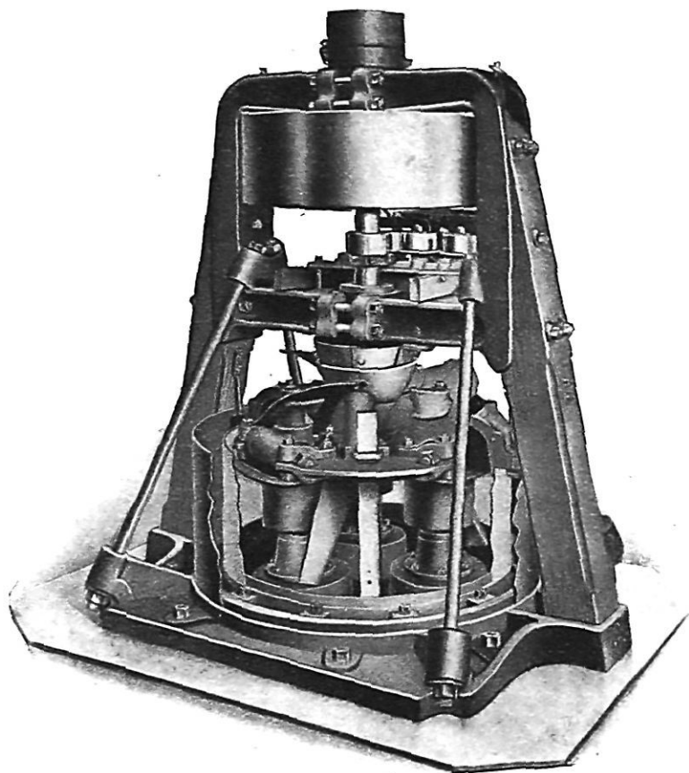
FIG. 6.—Bradley Three-Roll Mill.
