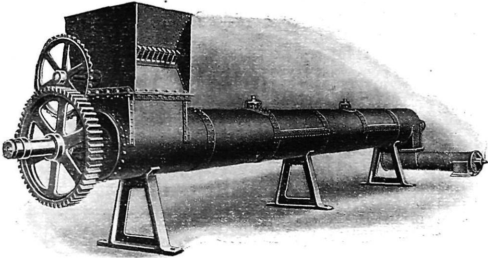
(A) Automatic Continuous Cooker or Digester.
