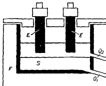
FIG. 6.—Furnace for Producing Silicon.
