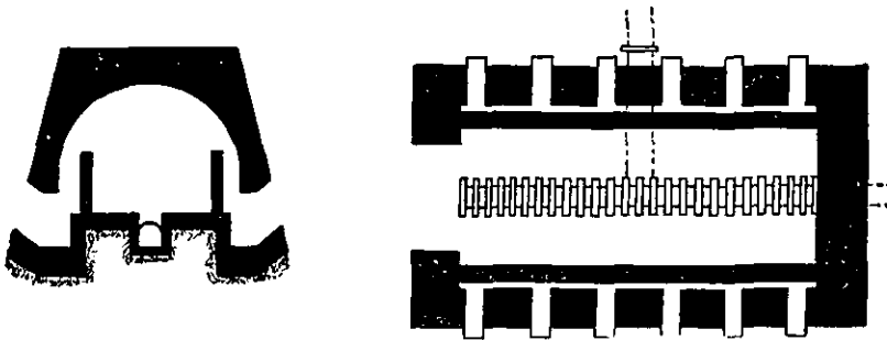
FIG. 17.—Cross Section and Plan of Down-Draught Kiln.
