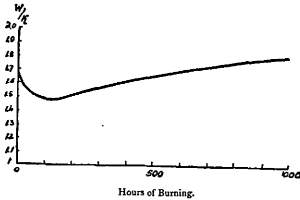
FIG. 8.—Variation in Consumption of Current of Tantalum Lamp.
