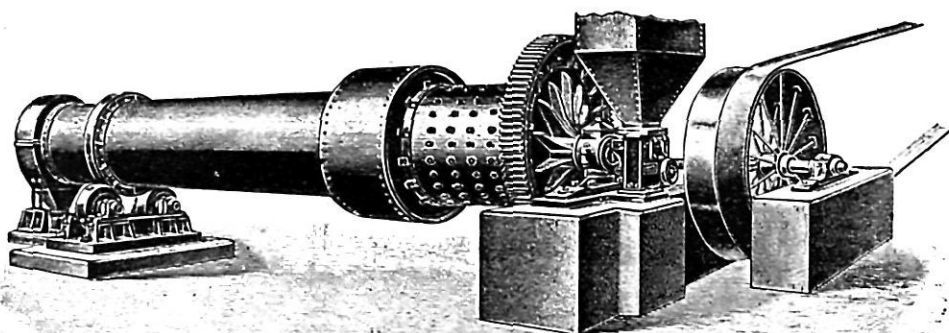
FIG. 17.—Löhnert's Compound Mill—External View.
