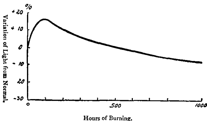
FIG. 7.—Variation of Luminosity of the Tantalum Lamp.
