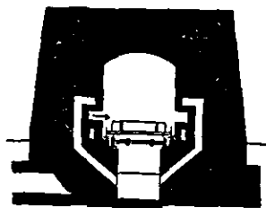
FIG. 16.—Cross Section of Tunnel Kiln.
