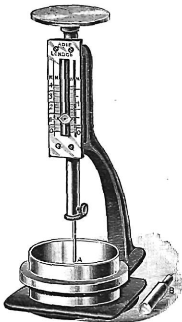
FIG. 35.—The Vicat Needle.
