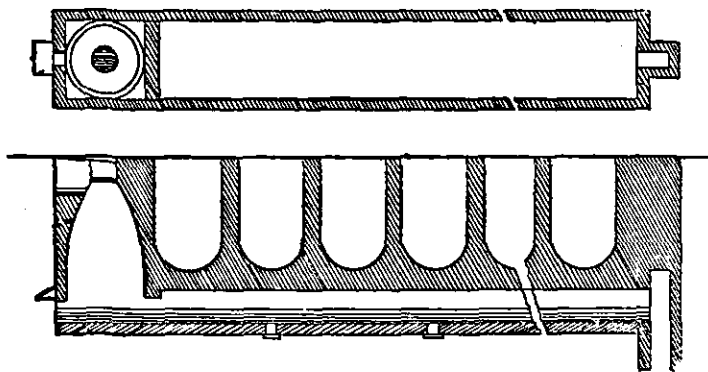
FIG. 25.—The Johnson Kiln.
