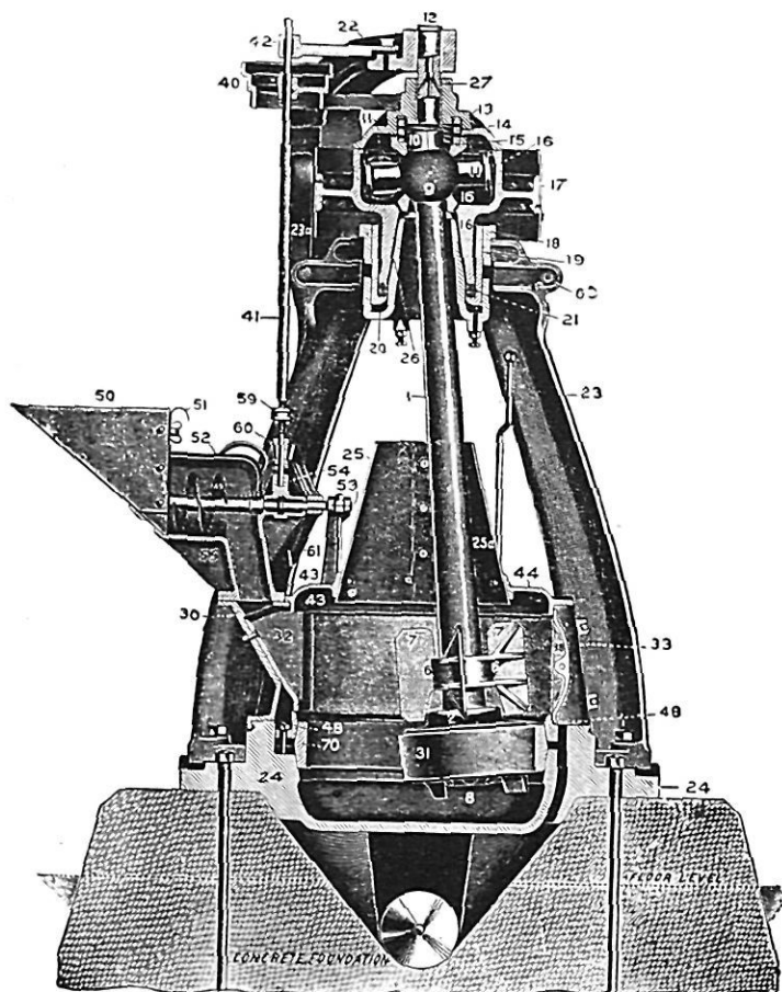
FIG. 15.—Section of Griffin Mill.
