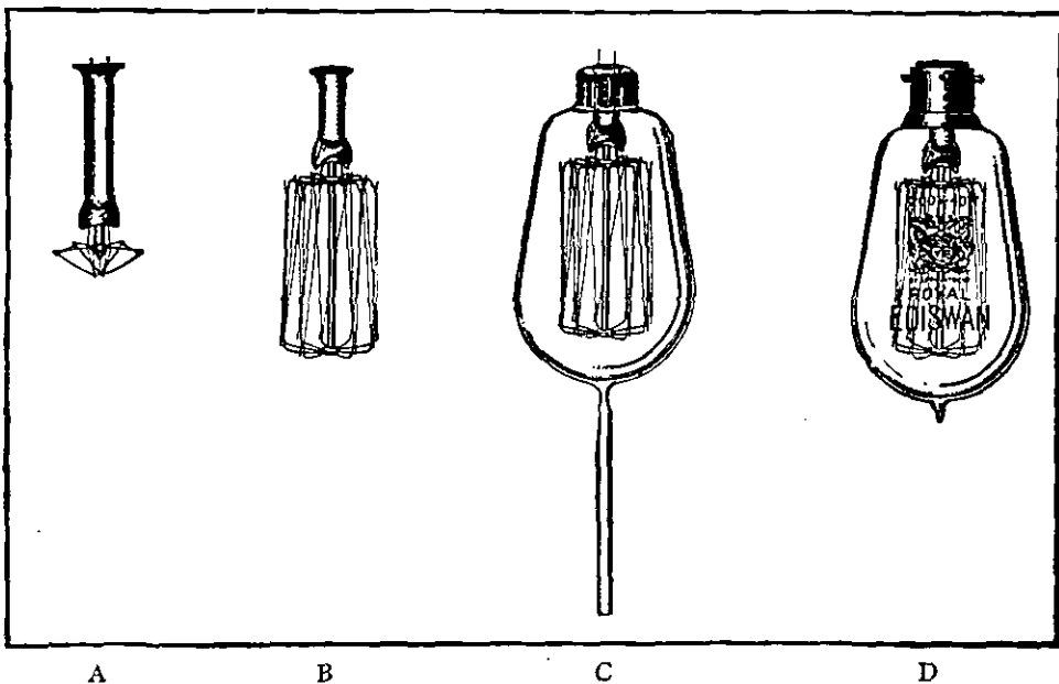
FIG. 19.—Stages in the Manufacture of a Metallic Filament Lamp.
