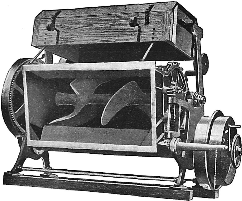
FIG. 12.—“Single-Blade Mixing Machine.” (Werner, Pfeiderer, & Perkins Ltd., Peterborough.)
