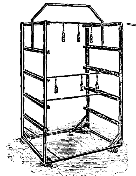
FIG. 19.—Movable Drying Crate for 500 Mantles, \frac{1}{4} Actual Size.
