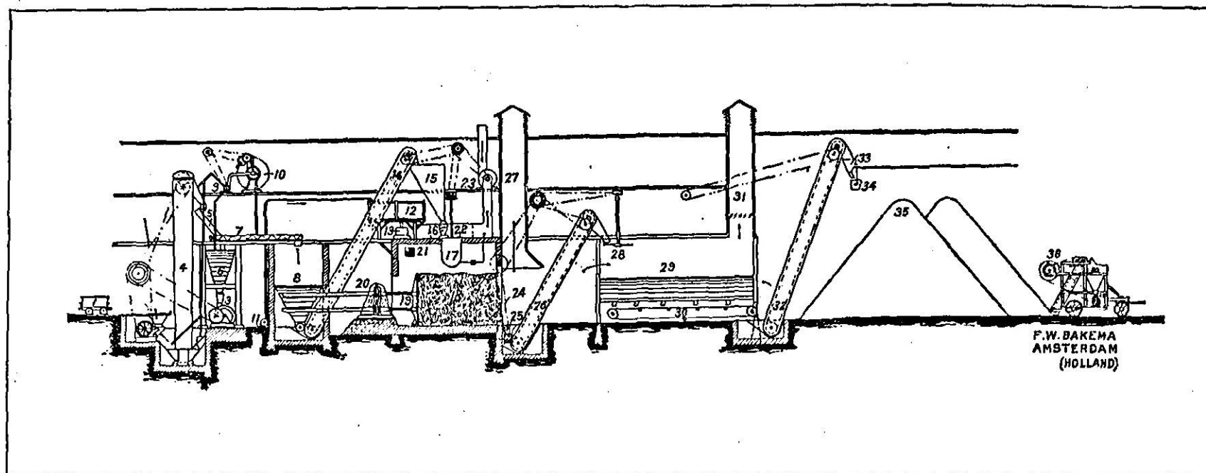
FIG. 1.—Complete Fertiliser Plant (see p. 31).
