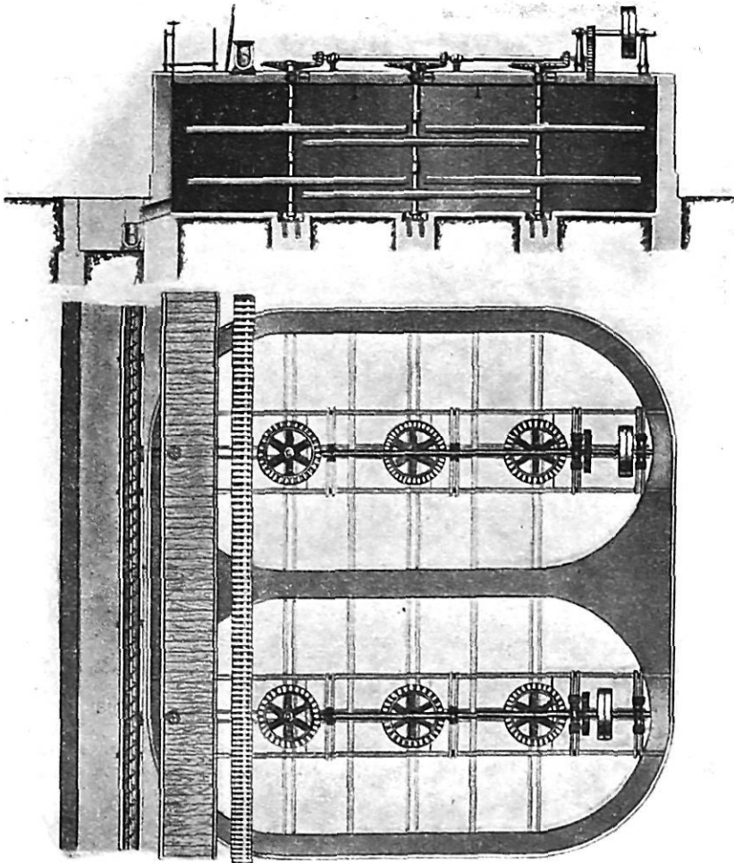
FIG. 10.—Mixer with Three Arms.
