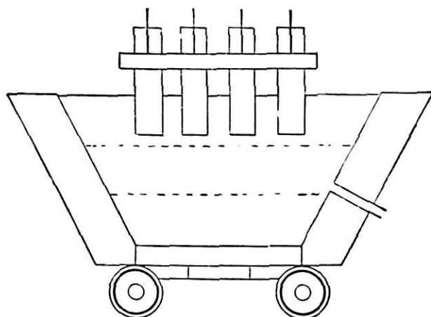
FIG. 9 -The Alby Carbide Furnace.
