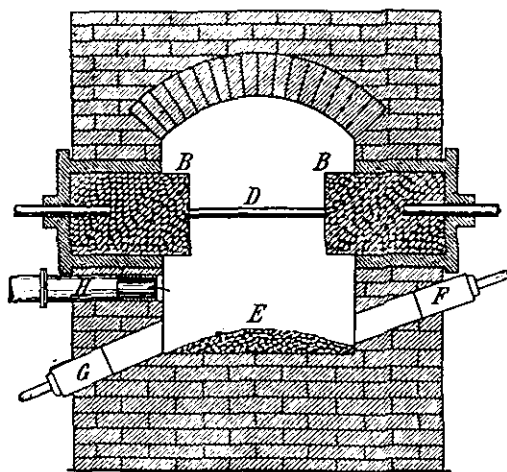
FIG. 3.—Phosphorus Furnace of the Electric Reduction Co.
