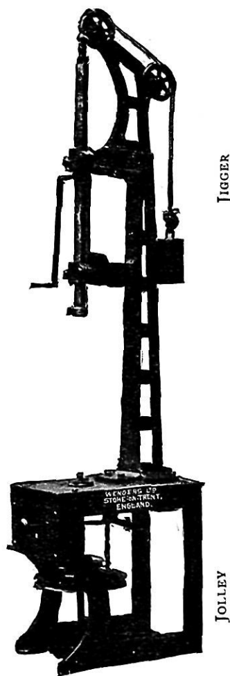
FIG. 6.—Vertical Jigger and Jolley.
