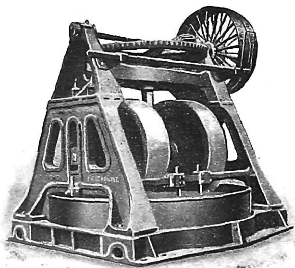
FIG. 3.—Edge-Runner Mill. (By courtesy of Messrs Sutcliffe, Speakman & Co. Ltd.)
