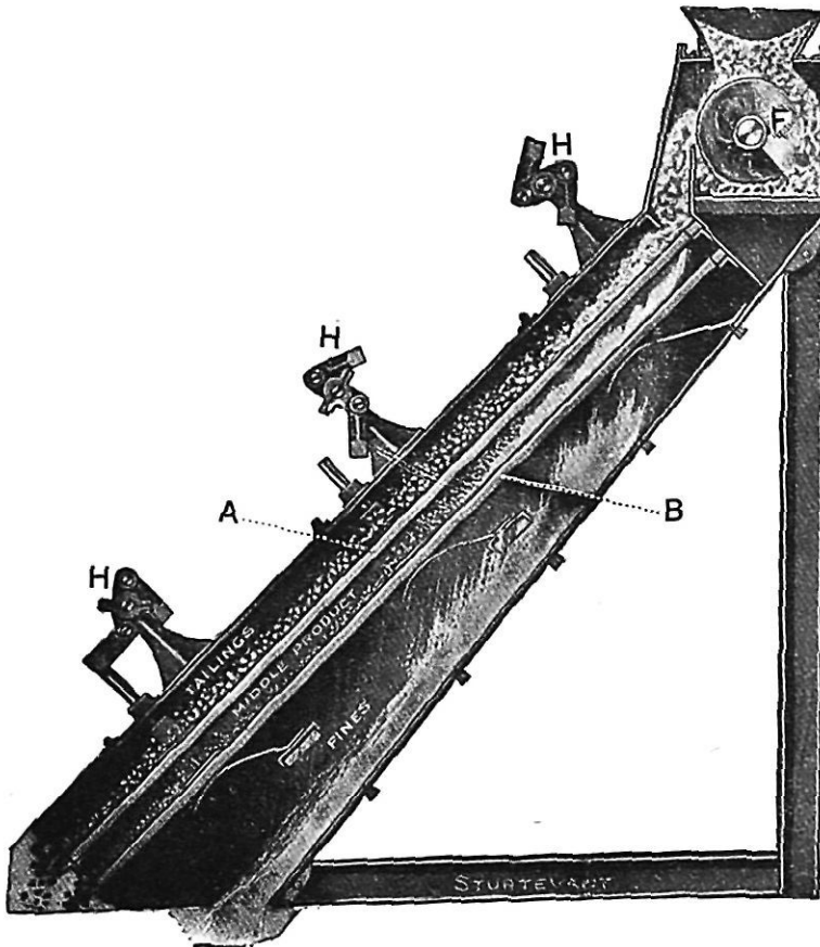
FIG. 8.—Sturtevant-Newaygo Separator. (Sturtevant Engineering Co. Ltd., London.)
