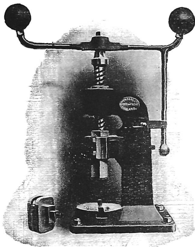
FIG. 11.—Screw Press for Small Ware. (By courtesy of Messrs Wengers Ltd.)
