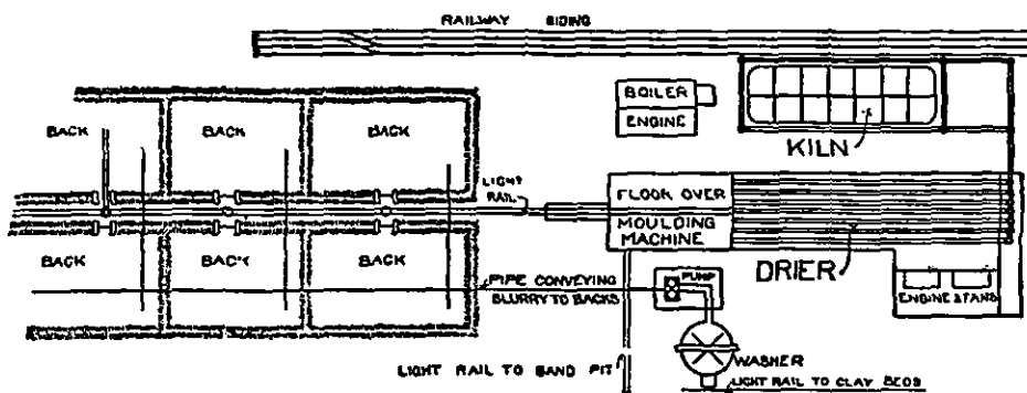
FIG. 2.—Arrangement of Washing Plant (after Middleton).
