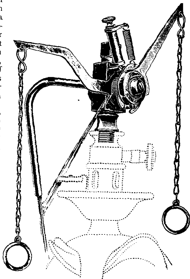
FIG. 23.—Automatic Lighter for Inverted Burners.
