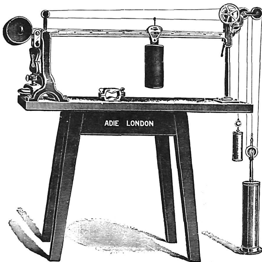
FIG. 33.—The Adie Testing Machine.
