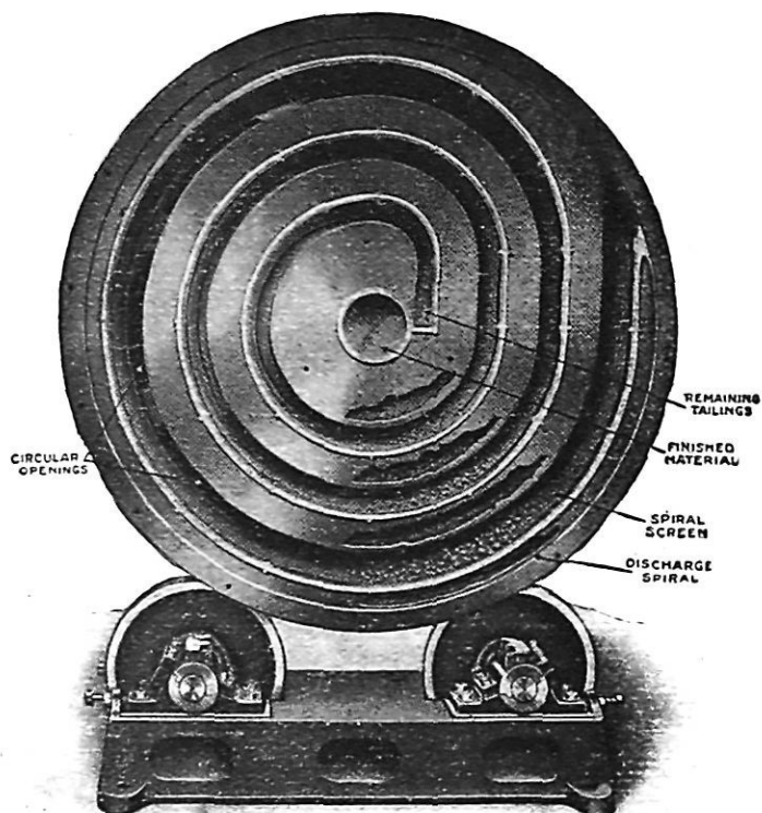
FIG. 3.—Abbé Ball Mill—Spiral Screen (open).
