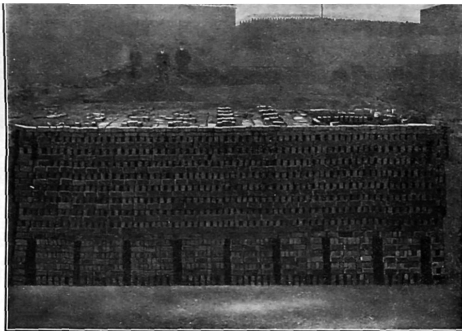
FIG. 15.—Archless Kiln.
