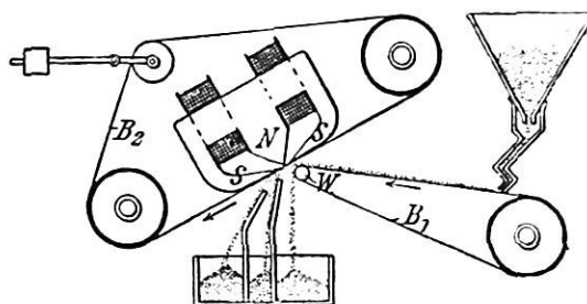
FIG. 4.—Wetherill Separator (Diagrammatic).
