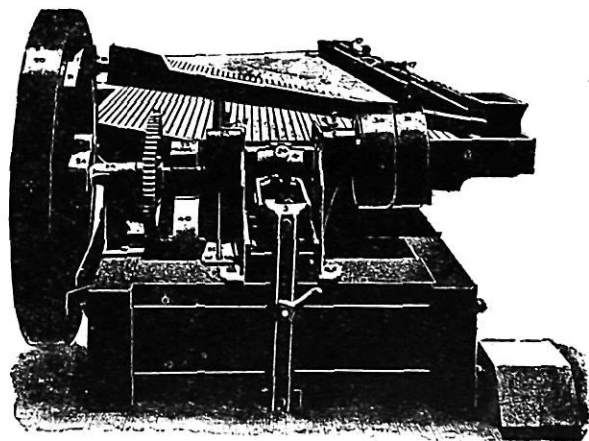
FIG. 1.—Movement End of Wilfley Table.
