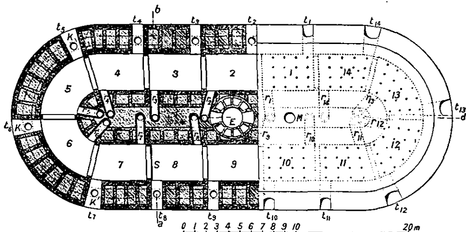
FIG. 20.—Plan of Hoffman Continuous Kiln.
