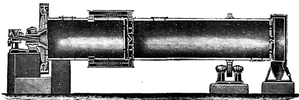
FIG. 18.—Löhnert's Compound Mill—Section.
