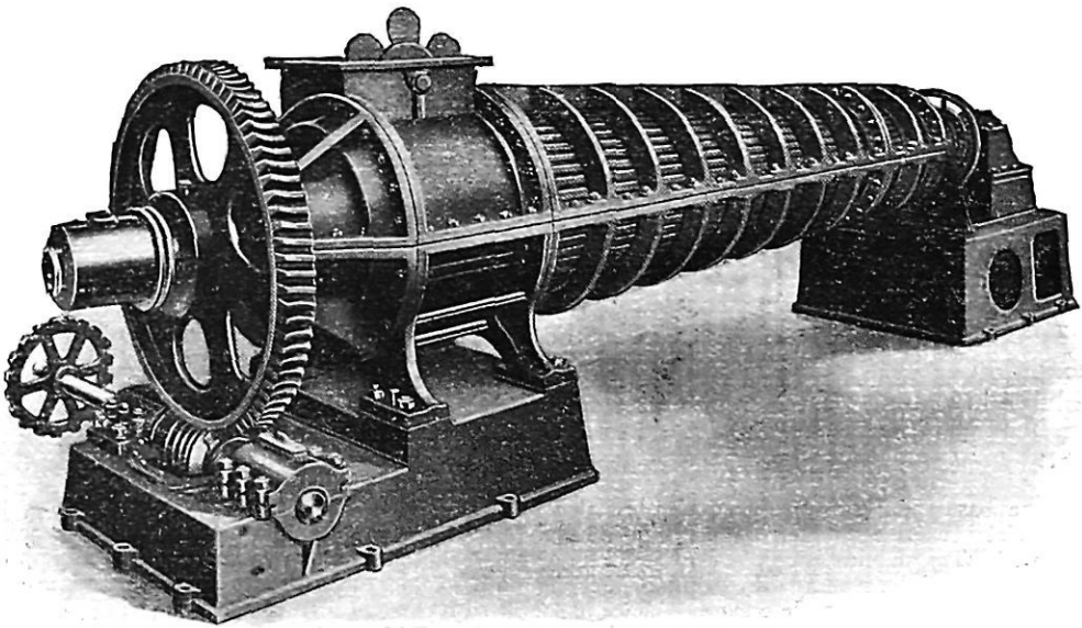
(B) Automatic Continuous Screw Press.
