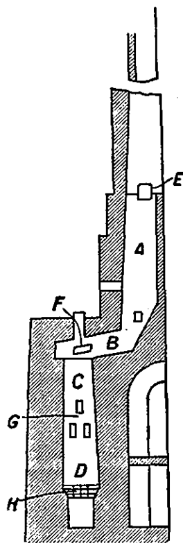
FIG. 26.—The Dietzsch Kiln.
