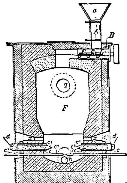
FIG. 1.—Vertical Section.
