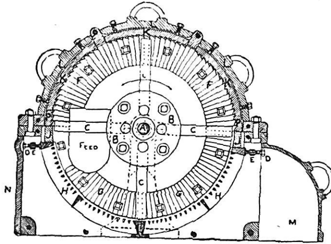
FIG. 7.—Section of Carter's Disintegrator. (J. Harrison Carter, London.)
