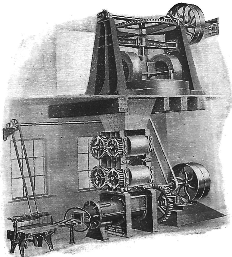
FIG. 7.—Plant for "Wire-Cut" Process. (By courtesy of Messrs J. Whitehead & Co. Ltd.)
