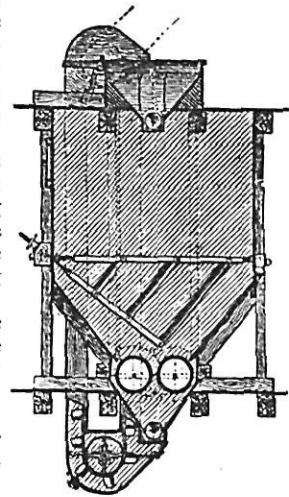
FIG. 19.—Mixing Silo
