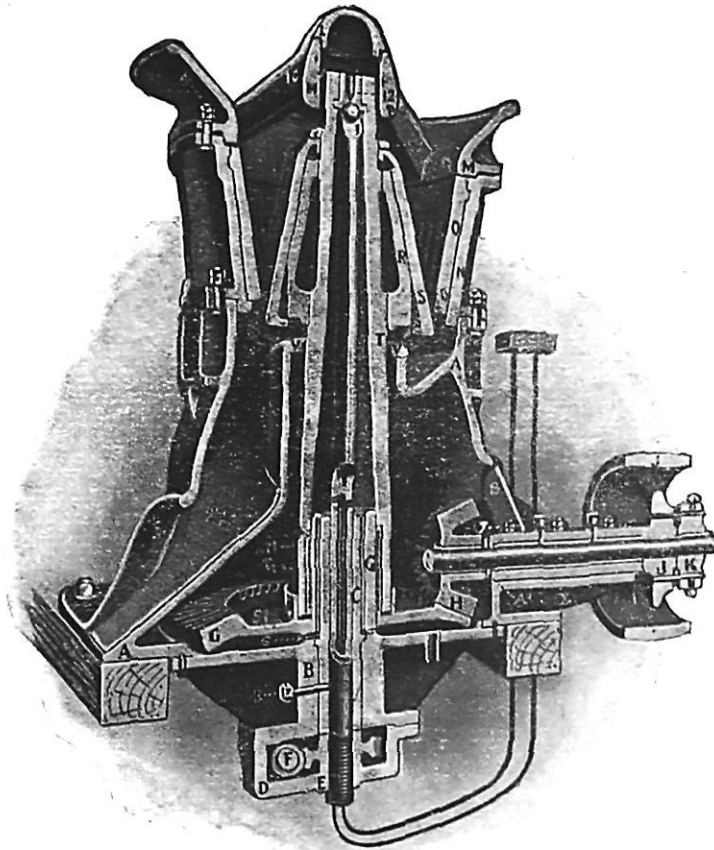
FIG. 12.—Hadfield's Gyratory Crusher.
