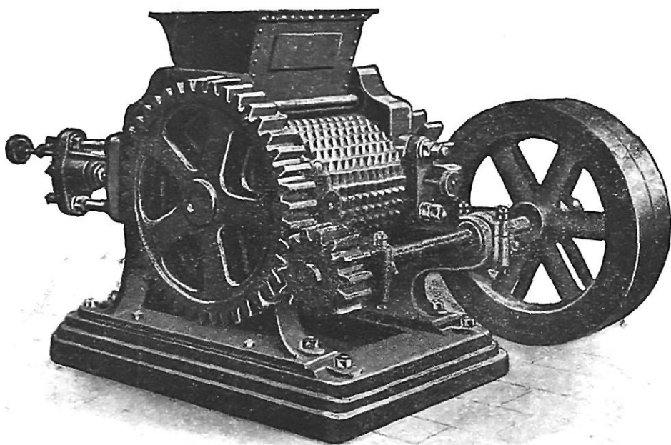
FIG. 13.—Roller Mill with Toothed Rolls.
