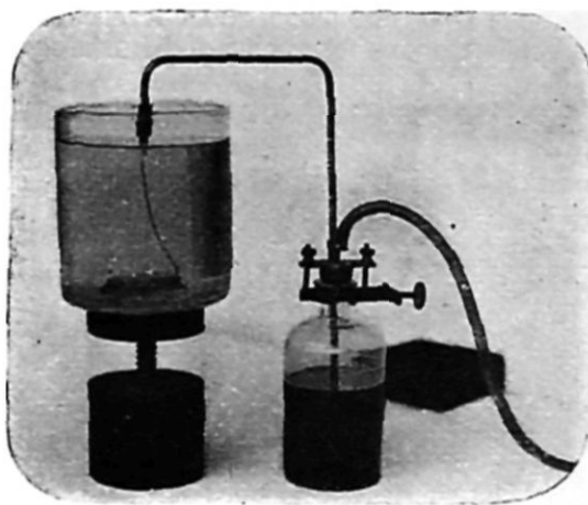
FIG. 3.—Squirting Carbon Filaments.
