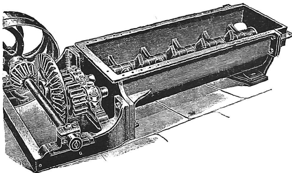
FIG. 4.—Open Mixer.
