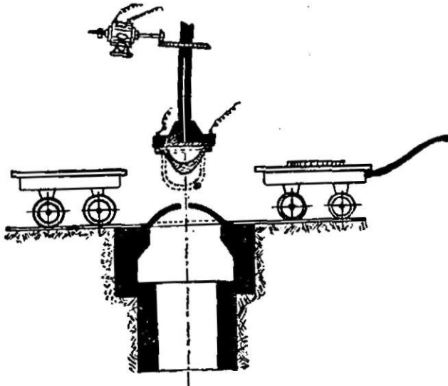
FIG. 10.—Sievert's Process.
