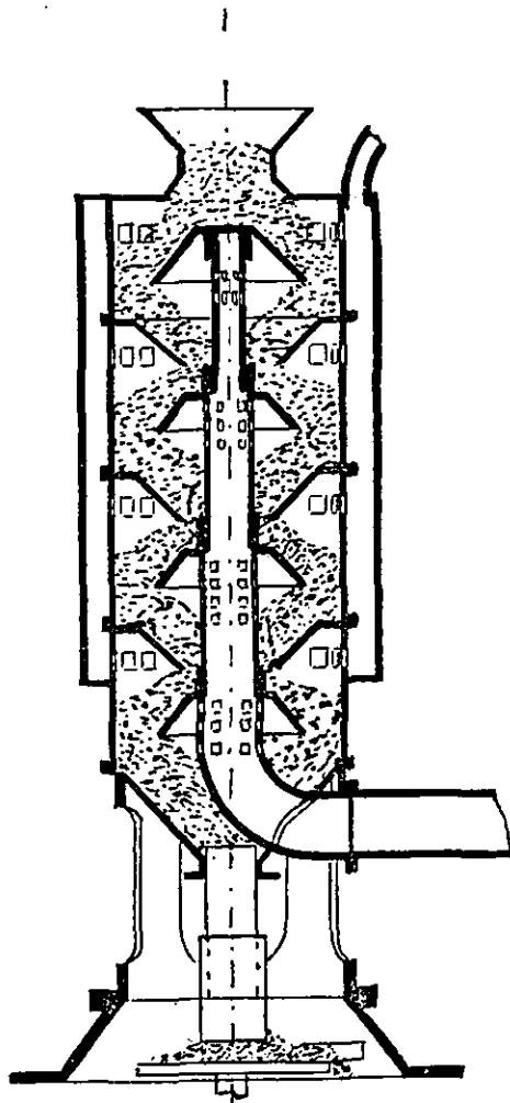
FIG. 24.—Mosser Vertical Cooler.
