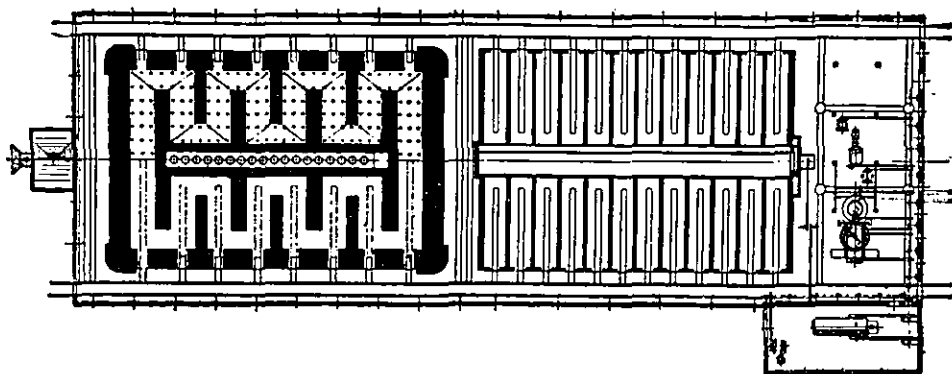
FIG. 21.—Plan of Bühler Continuous Kiln and Drier.
