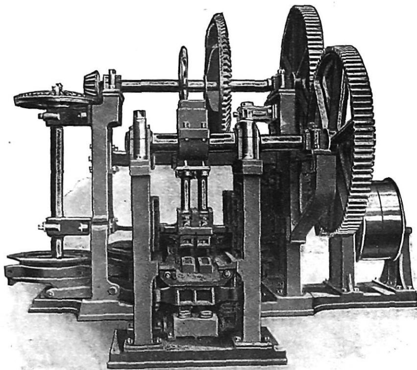
FIG. 10.—Machine for Making Bricks by the Stiff-Plastic Process.
