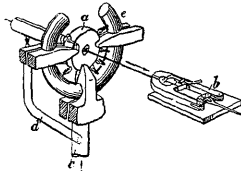
FIG. 16.—Heated Drawplate.
