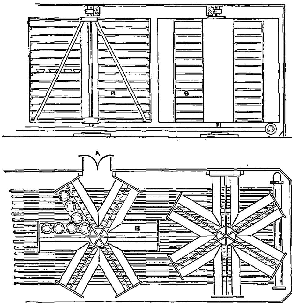
FIG. 12.—Section and Plan of Drying Stove.
