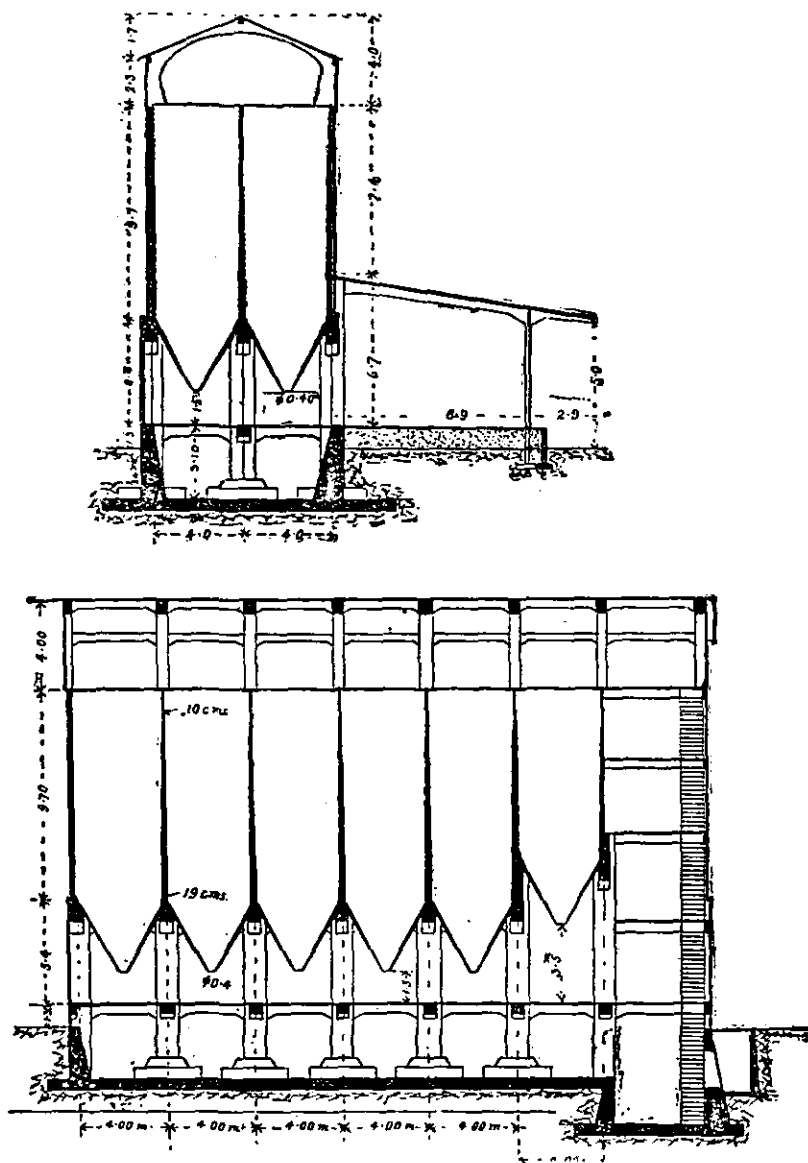
FIG. 28.—Silos with Hopper-Shaped Bottoms.
