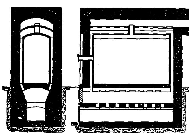
FIG. 1.—Sections of Muffle Kiln.
