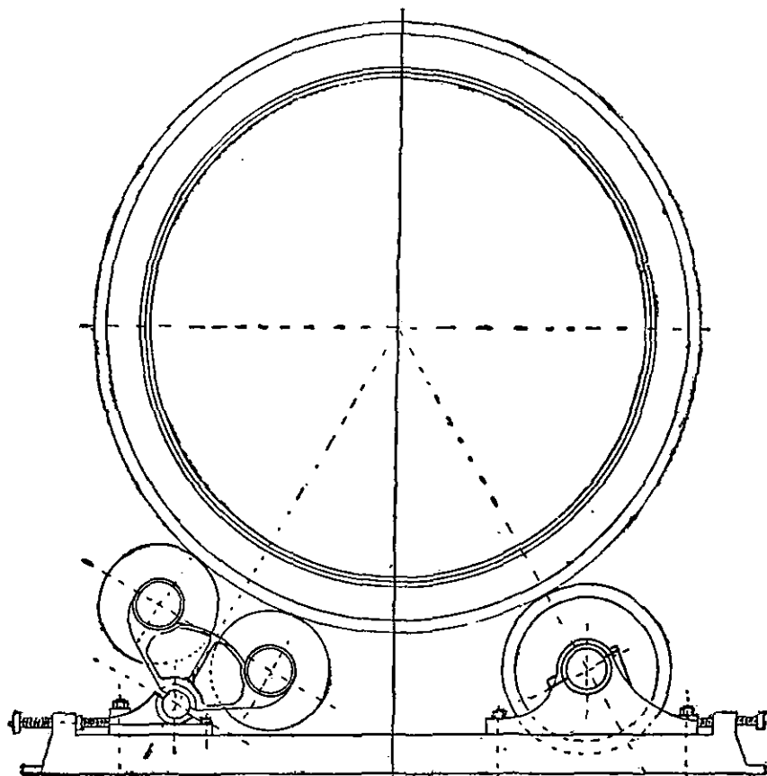
FIG. 22.—Forms of Bearing for Rotary Kiln.
