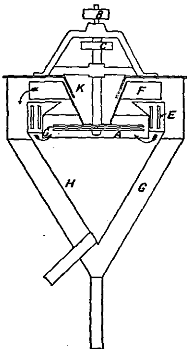
FIG. 9.—Section of an Air Separator.
