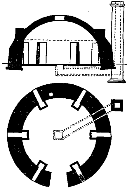
FIG. 16.—Cross Section of Round Down-Draught Kiln.
