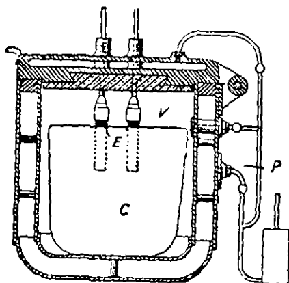
FIG. 5.—Alundum Furnace of Pettigrew and Gerbel-Strover.
