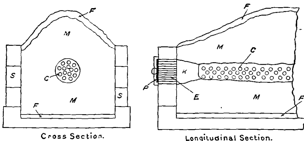
FIG. 1.—Carborundum Furnace.
