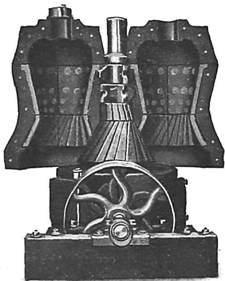
FIG. 6.—Cracker of the Coffee-Mill Type. A rotary fine crusher supplied by the Sturtevant Engineering Co. Ltd., London.
