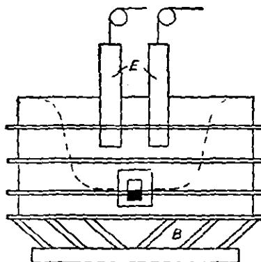
FIG. 8.—Modern Ferro-Silicon Furnace.
