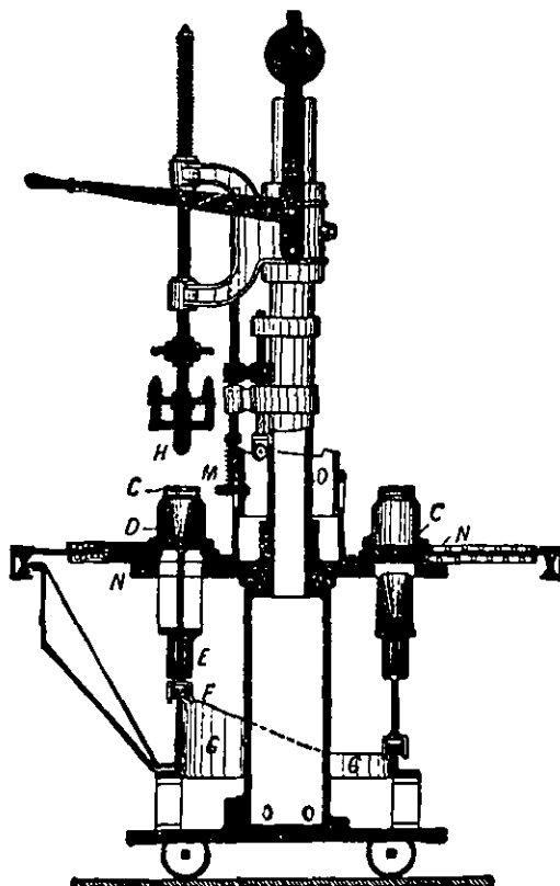
FIG. 8.—Brühler's Glass Machine.
