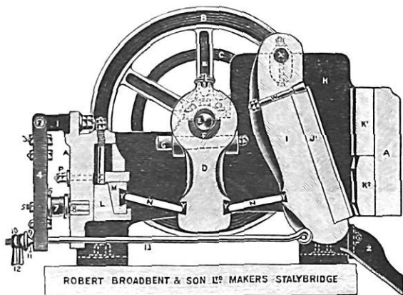
FIG. 11.—Section of Broadbent's Improved Blake Stonebreaker.
