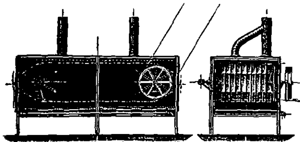
FIG. 13.—Drying Chamber.
