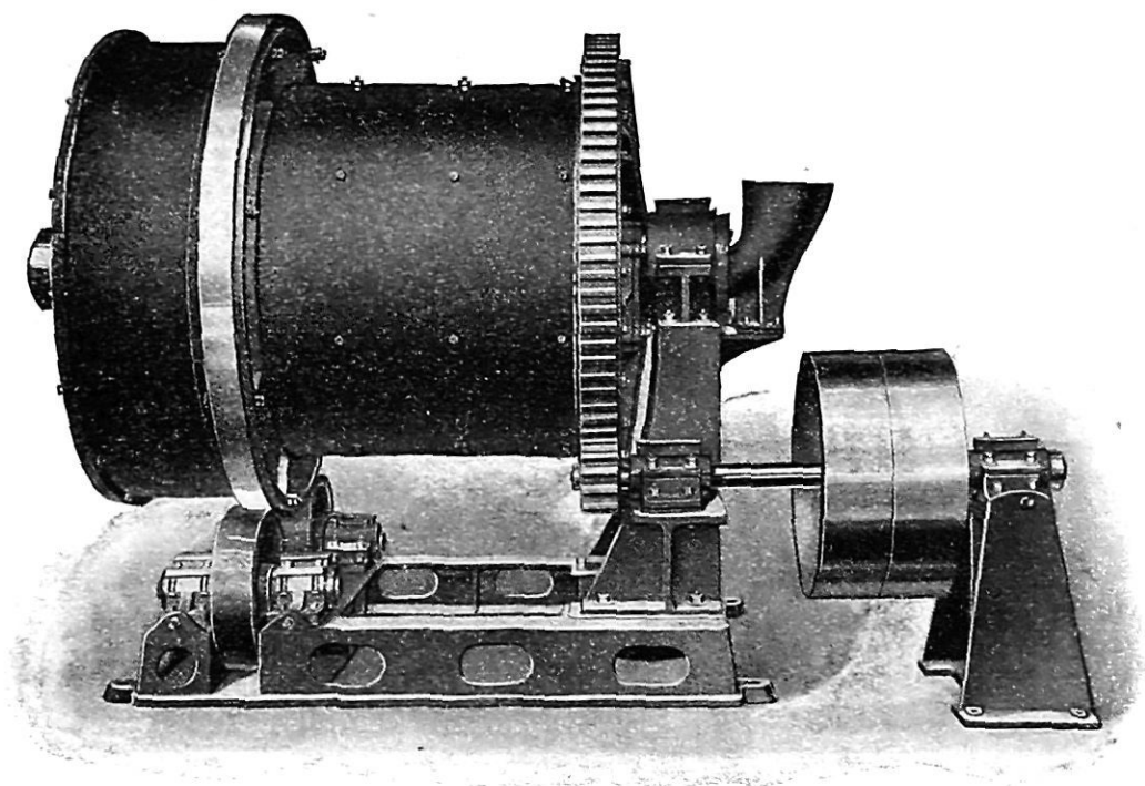
FIG. 2.—Abbé Ball Mill. (The Abbé Engineering Co., New York.)
