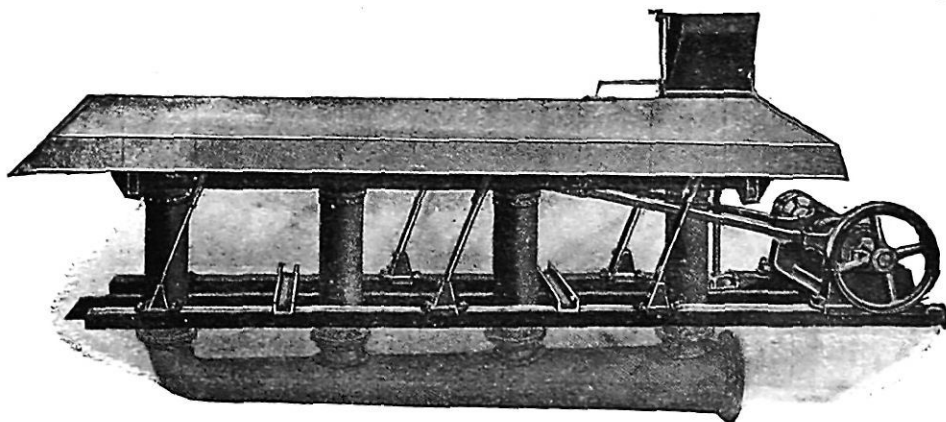
FIG. 2.—Sutton-Steele Dry Concentrating Table.
