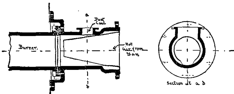
FIG. 23.—Coal Dust Burner Attachment.
