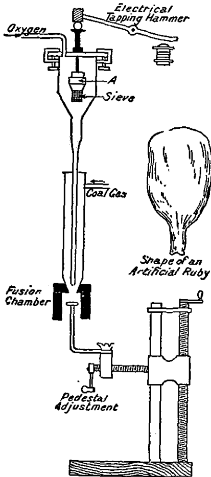
FIG. 1.—Verneuil's Blowpipe for Artificial Rubies and Sapphires.
