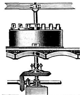
FIG. 1.—Wet Grinding Mill.
