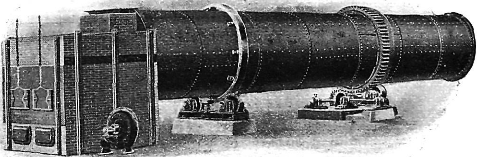
(C) Direct Heat Rotary Drier (with ring gear).
