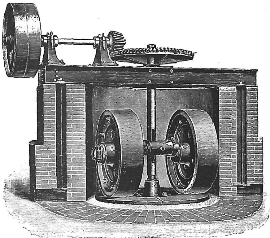
FIG. 8.—Wet Edge-Runner.
