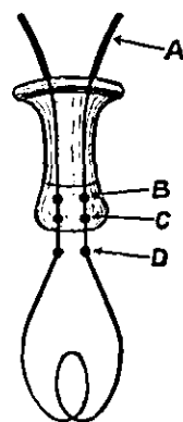
FIG. 2. Connections between Filament and Leading-in Wires.
