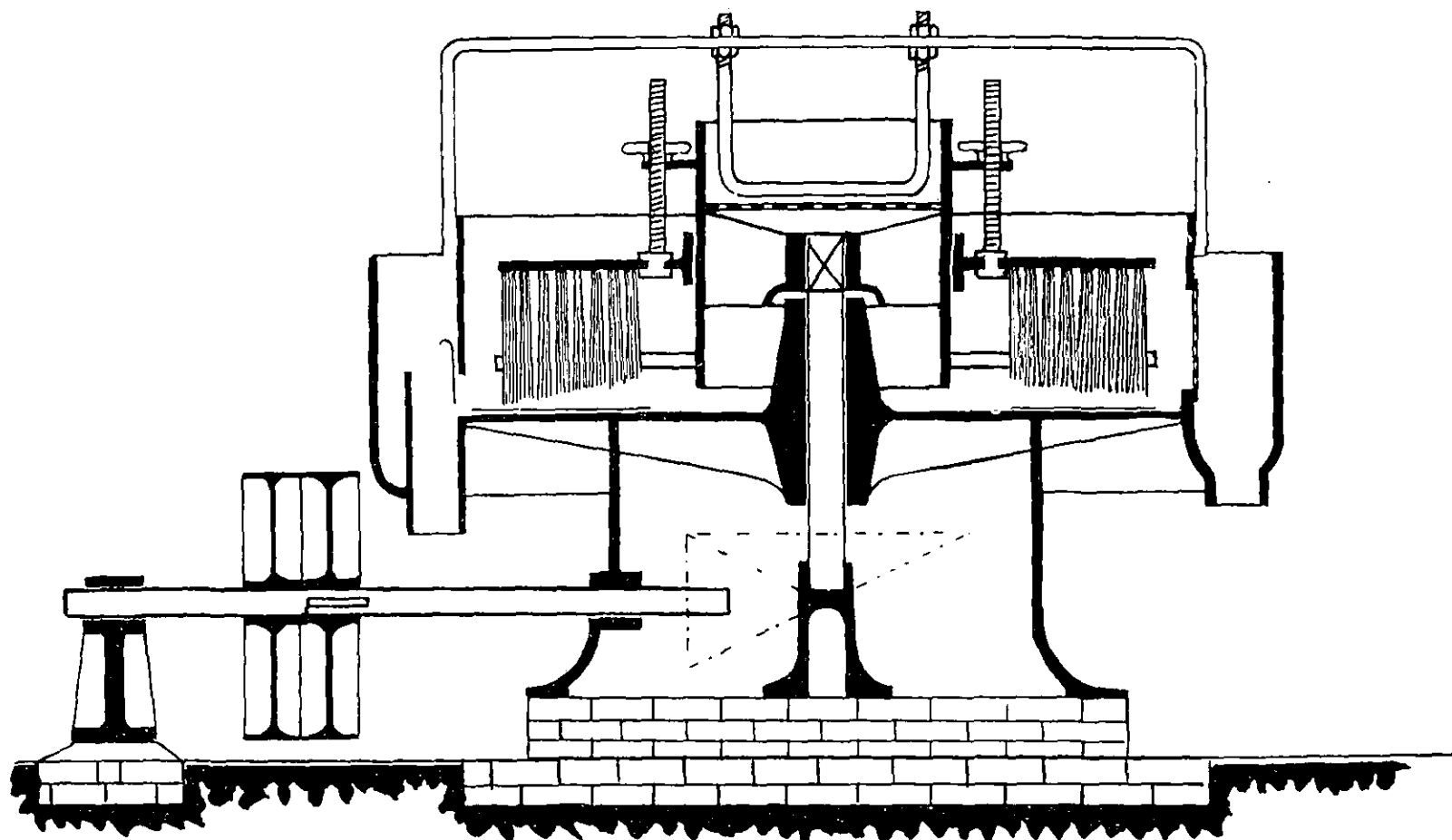
FIG. 9.—Clarke's Mill.
