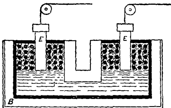
FIG. 7.—Keller Furnace.
