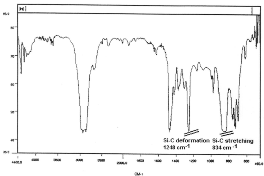
Figure 5.3 IR spectrum of ethylene-vinyltrimethylsilane copolymer
