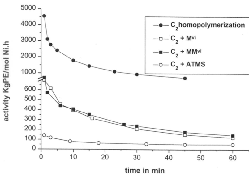
Figure 5.6 Kinetic profile of ethylene polymerization using the catalyst system DABANiBr 2 /MAO in the presence of comonomers
