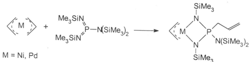
Scheme 1.5 Ni and Pd catalysts with aminobis(imino)phosphorane ligand
