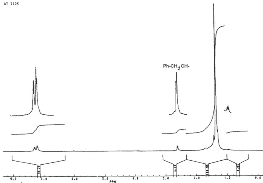
Figure 4.7 ^1\text{H} NMR spectrum of ethylene-allylbenzene copolymer
