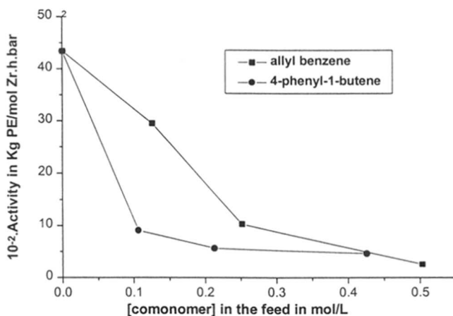
Figure 4.8 Effect of comonomer concentration on catalyst activities for ethylene polymerization (catalyst system \text{Cp}_2\text{ZrCl}_2/\text{MAO} )
