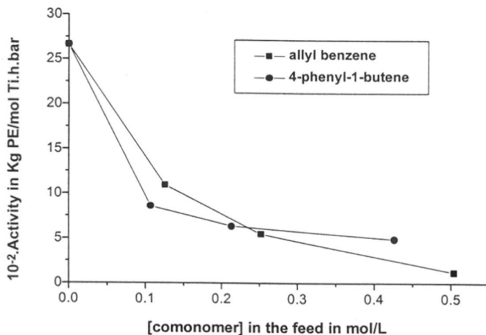
Figure 4.10 Effect of comonomer concentration on catalyst activities for ethylene polymerization (catalyst system \text{Me}_2\text{SiCp}_2\text{TiCl}_2/\text{MAO} )
