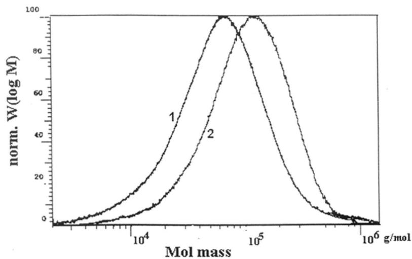
Figure 6.11 GPC curves of poly (ethylene)s synthesized using different TIBAL/Fe ratios (1) 1500 and (2) 1000
