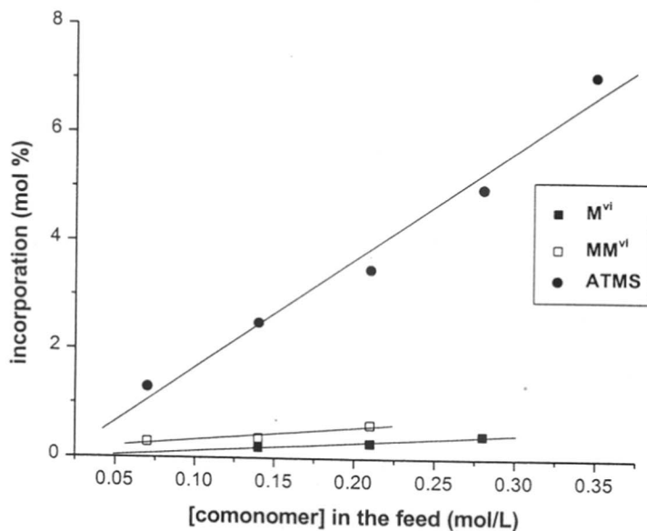
Figure 5.9 Effect of comonomer feed on copolymer composition
