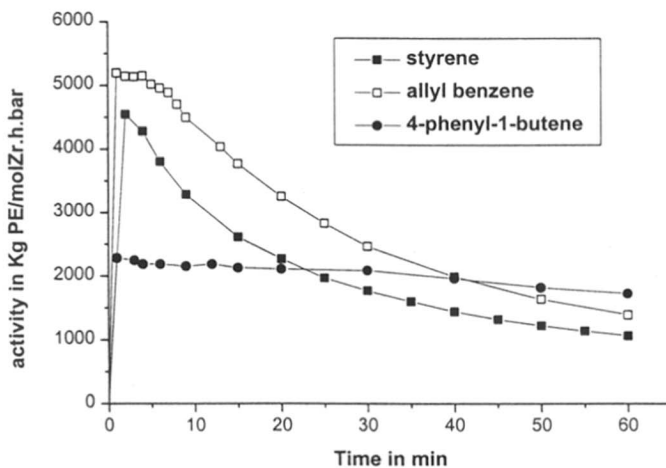
Figure 4.3 Kinetic profile of ethylene polymerization using Me_2SiCp_2ZrCl_2 in the presence of different comonomers
