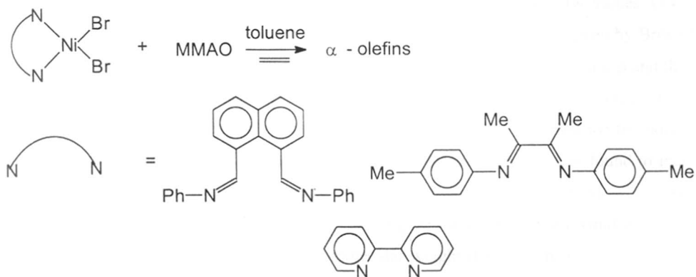
Scheme 1.9 Oligomerization of ethylene using Ni (diimine) complexes
