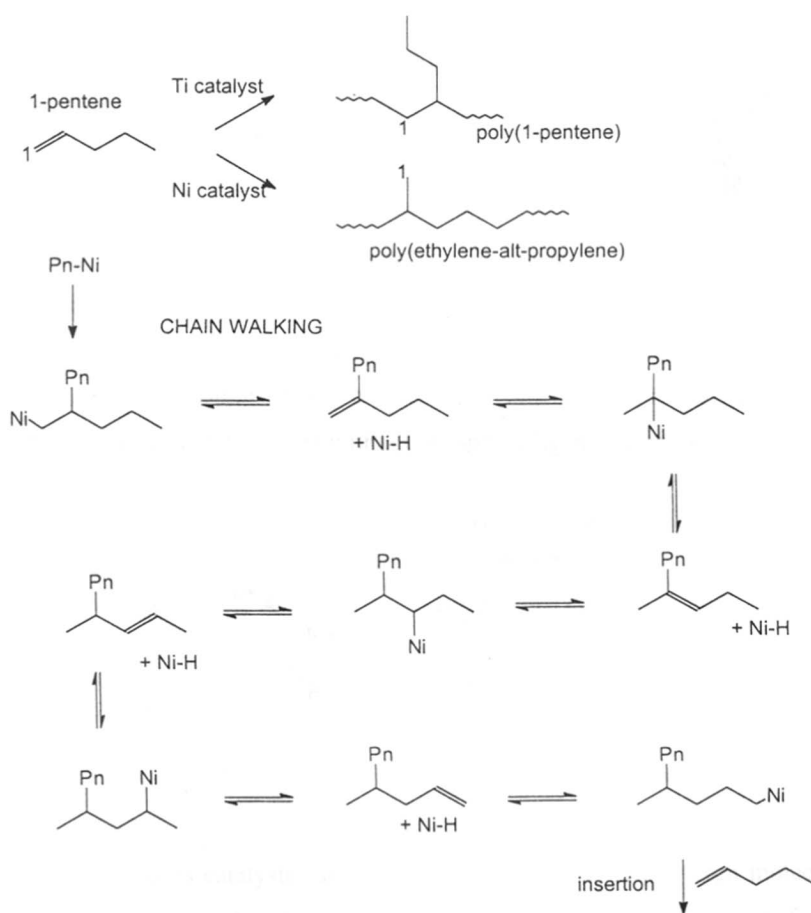
Scheme 1.6 Chain walking mechanism
