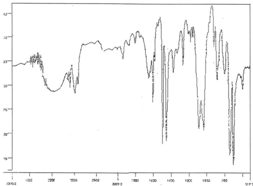
Figure 4.1 IR spectrum of polyallylbenzene prepared with \text{Cp}_2\text{ZrCl}_2/\text{MAO}
