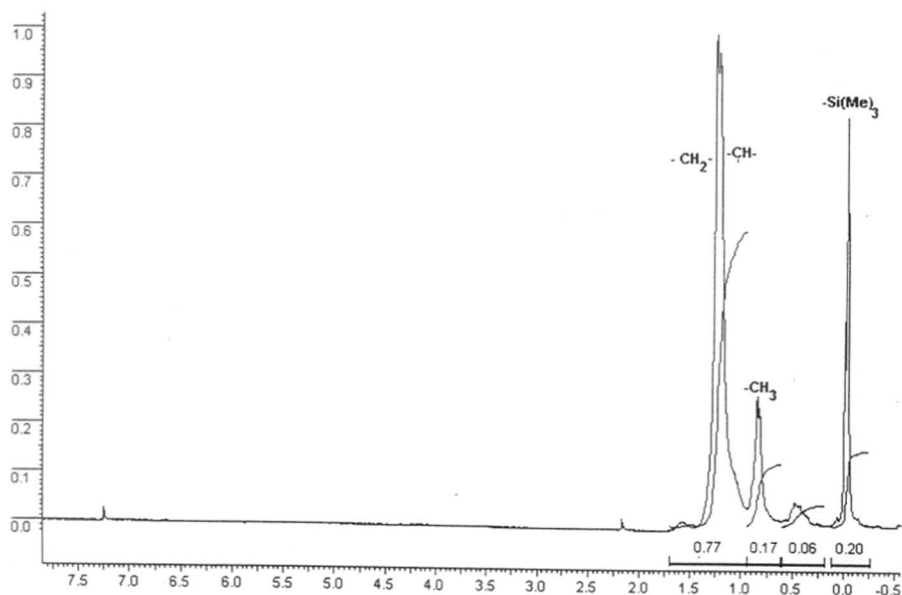
Figure 5.8 ^1\text{H} NMR spectrum of copolymer of ethylene with ATMS (Table 5.8; Entry 9)
