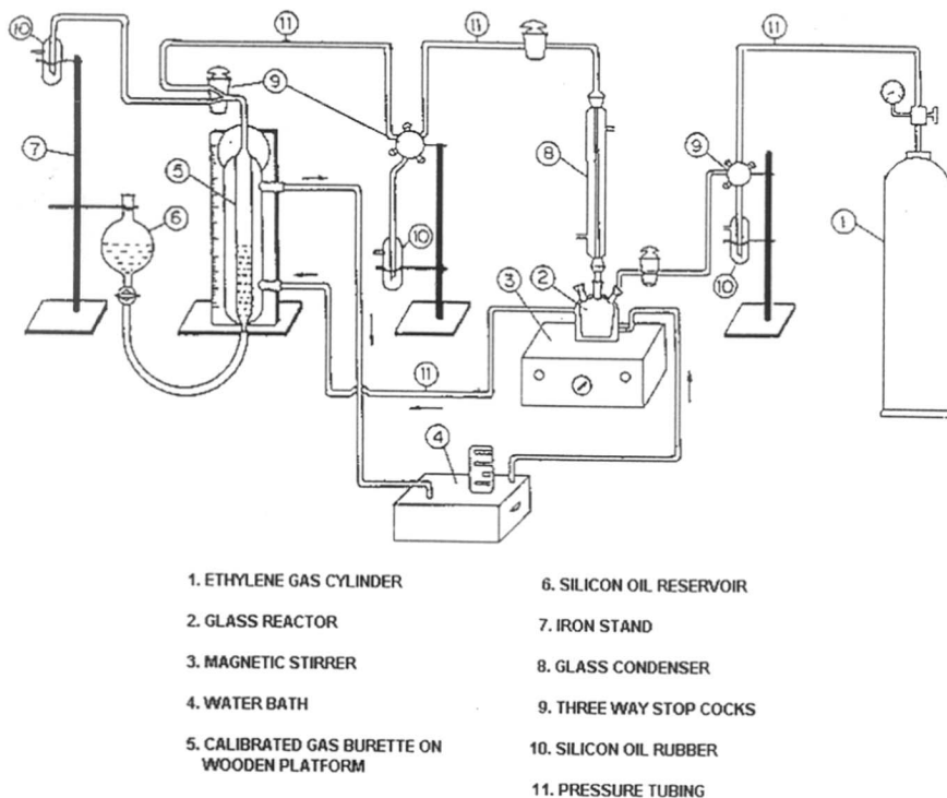
Figure 3.1 Ethylene polymerization set-up at one atmosphere pressure
