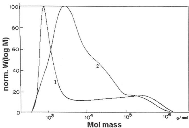
Figure 6.15 GPC curves of poly(ethylene)s synthesized using different catalyst concentrations (TMA); (1) 5 \times 10^{-6} and (2) 1.1 \times 10^{-6}
