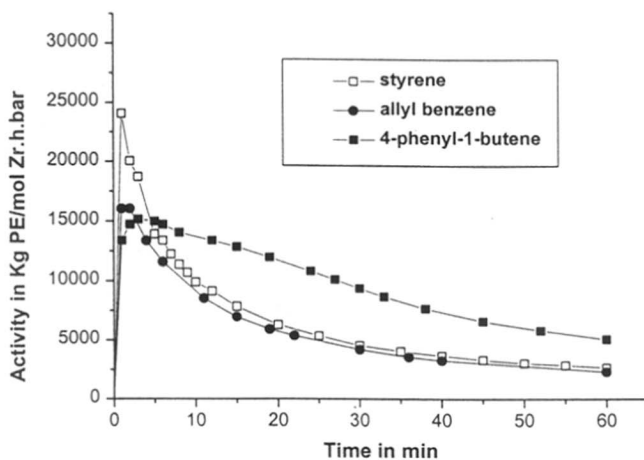
Figure 4.2 Kinetic profile of ethylene polymerization using Cp_2ZrCl_2 in the presence of different comonomers
