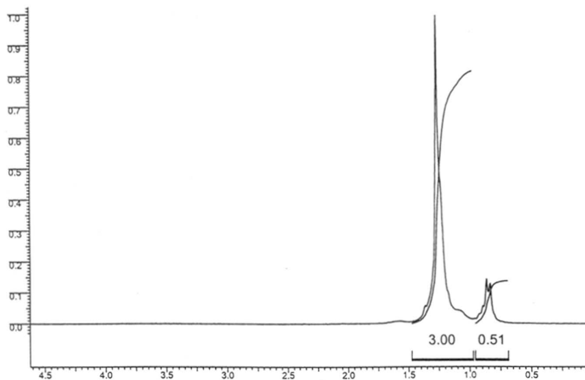
Figure 6.21 1 H NMR spectrum of poly(ethylene): (DABAn)NiBr 2 /DEAC (Table 6.7, Entry 11)
