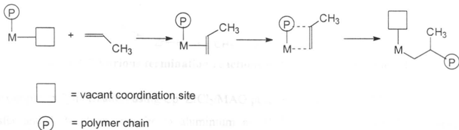
Scheme 1.1 Cossee mechanism for Ziegler-Natta polymerization
