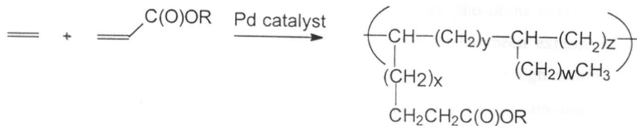
Scheme 1.11 Copolymerization of ethylene with functional monomers
