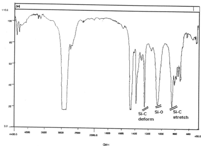
Figure 5.7 IR spectrum of ethylene- MM^{vi} copolymer
