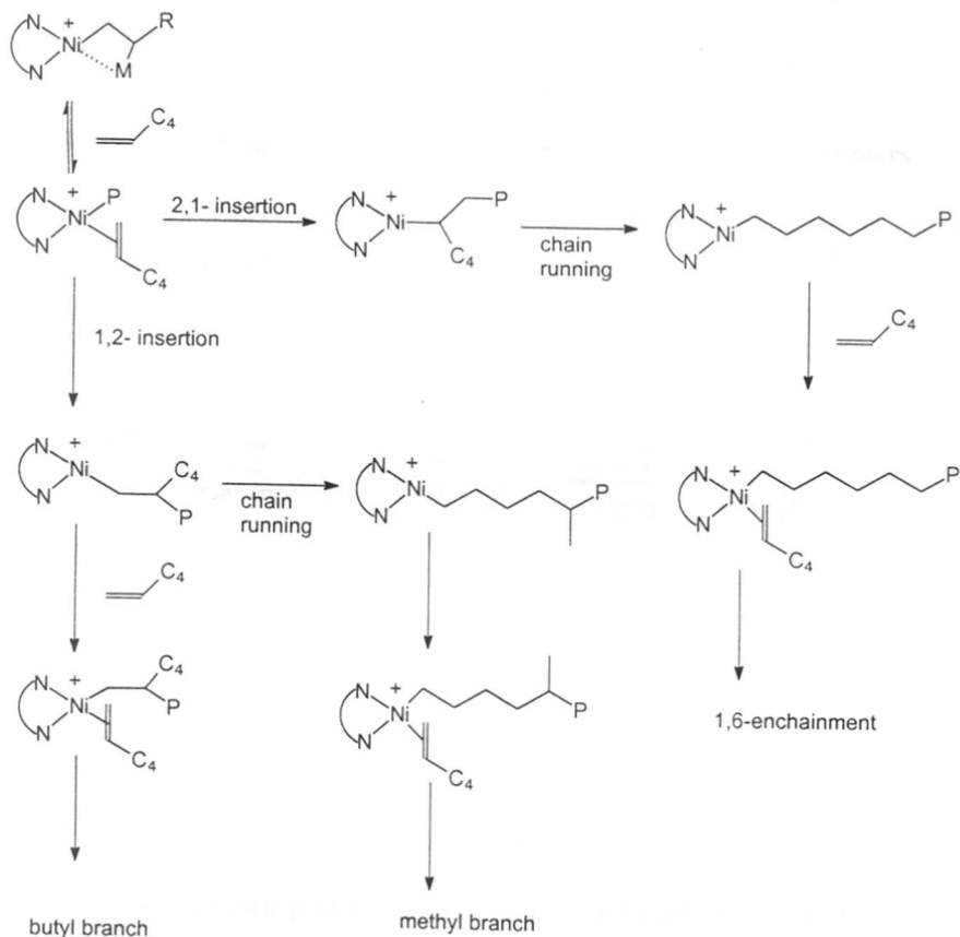
Scheme 1.10 Mechanism of 1,ω polymerization of α-olefins
