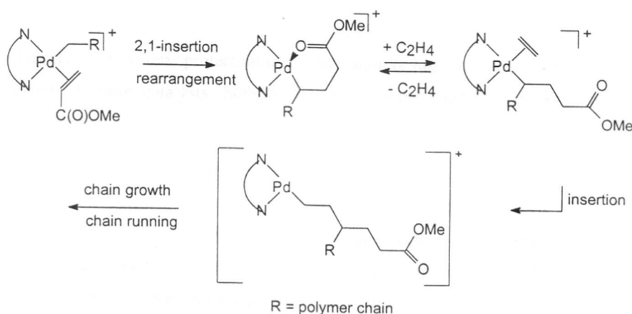
Scheme 1.12 Mechanistic pathway for the formation of poly(ethylene-co-acrylates)
