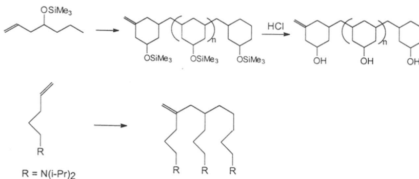
Scheme 1.3 Polymerization of functional monomers
