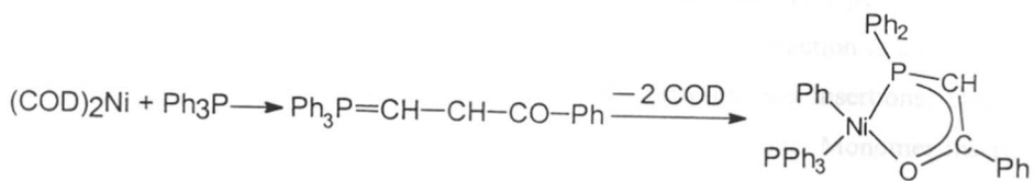
Scheme 1.4 Oligomerization /polymerization catalyst
