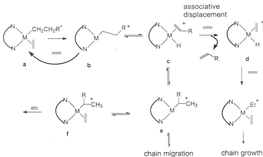
Scheme 1.8 Mechanism of ethylene polymerization
