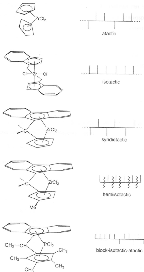
Figure 1.1 Correlation of metallocene structure to polypropylene structure
