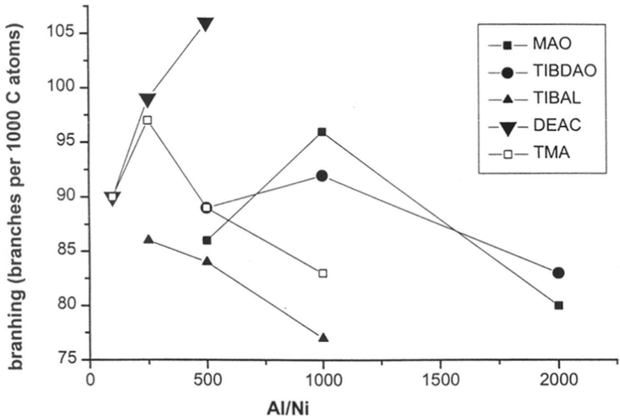
Figure 6.24 Effect of Al/Ni ratio on branching
