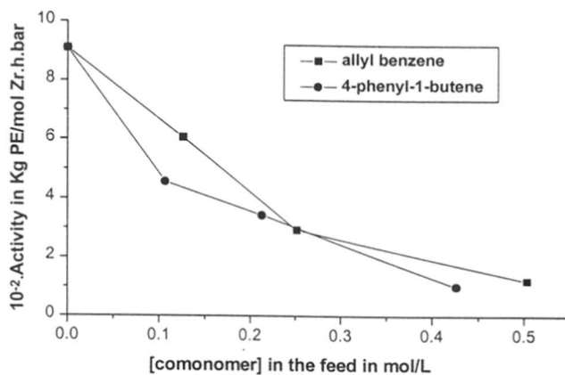
Figure 4.9 Effect of comonomer concentration on catalyst activities for ethylene polymerization (catalyst system \text{Me}_2\text{SiCp}_2\text{ZrCl}_2/\text{MAO} )
