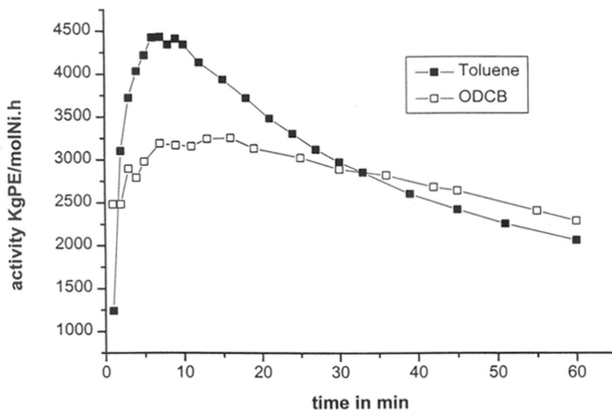
Figure 6.27 Kinetic profile of ethylene polymerization using different solvents
