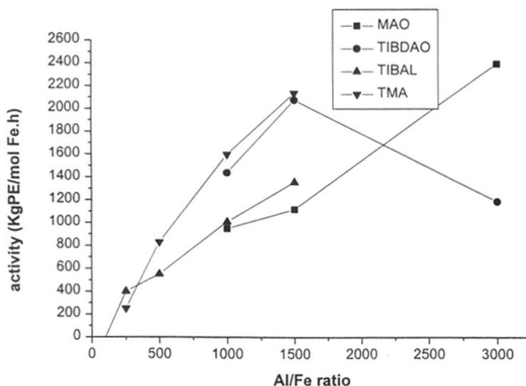
Figure 6.5 Effect of Al/Fe ratio on catalyst activity
