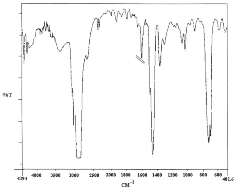
Figure 4.5 IR spectrum of ethylene-allyl benzene copolymer
