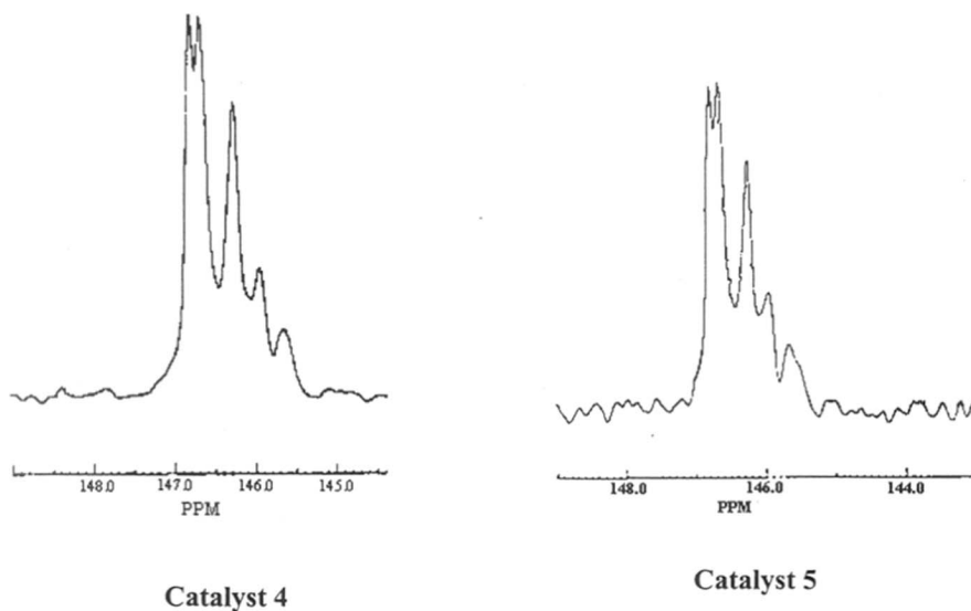
Figure 4.13 ^{13}\text{C} spectra of partially isotactic rich polystyrene
