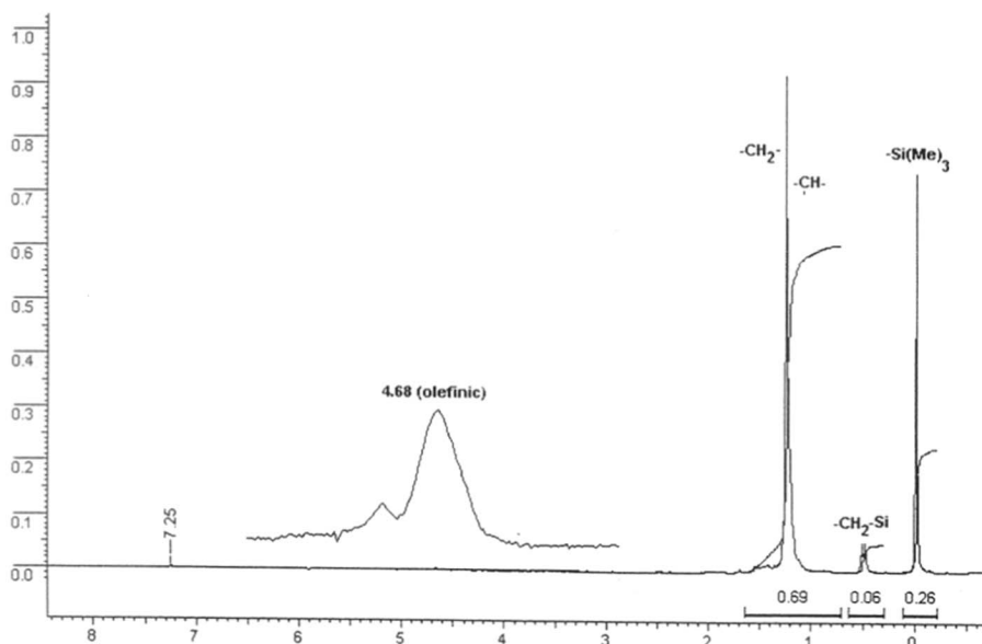
Figure 5.5 ^1\text{H} NMR spectrum of ethylene-ATMS copolymer synthesized with metallocene (Table 5.3 Entry 4)
