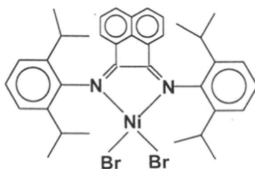
Figure 6.20 Structure of the Ni(diimine) catalyst, (\text{DABAn})\text{NiBr}_2
