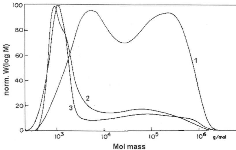
Figure 6.14 GPC curves of poly(ethylene)s synthesized using different catalyst concentrations / (MAO); (1) 1.1 \times 10^{-6} , (2) 5 \times 10^{-6} and (3) 10 \times 10^{-6}
