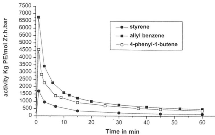
Figure 4.4 Kinetic profile of ethylene polymerization using \text{Me}_2\text{SiCp}_2\text{TiCl}_2 in the presence of different comonomers
