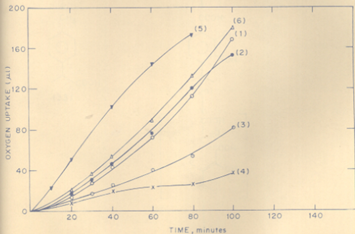
FIG. XXXIII. OXIDATION OF VARIOUS AROMATIC ACIDS BY P-CYMENE GROWN CELLS (1.44 mg. DRY WEIGHT/FLASK).
