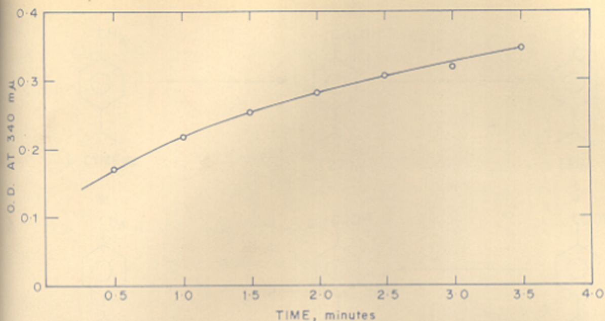
FIG. XL. ACTIVITY OF ALDEHYDE DEHYDROGENASE IN PRESENCE OF CUMIC ALDEHYDE.
