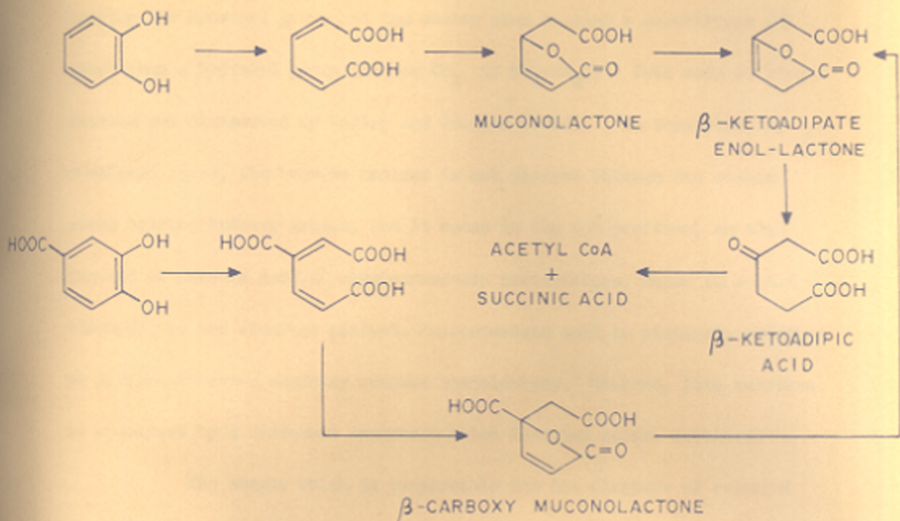
FIG. III. METAPYROCATCHASE-TYPE RING CLEAVAGE OF CATECHOL AND PROTOCATECHUIC ACID
