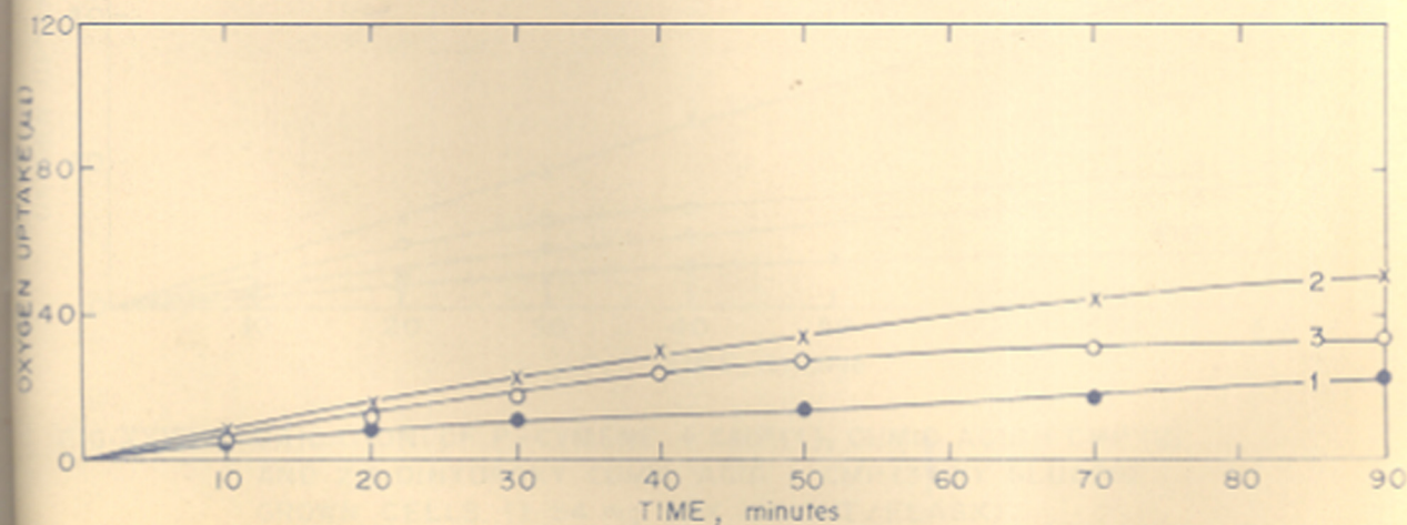
FIG. XXXI b. OXIDATION OF P-CYME + CMP (1) CUMIC ACID + CMP (2) AND 2,3-DIHYDROXY CUMIC ACID + CMP (3) BY 2,3 DIHYDROXY CUMIC ACID GROWN CELLS (1.46 mg. DRY WEIGHT / FLASK).
