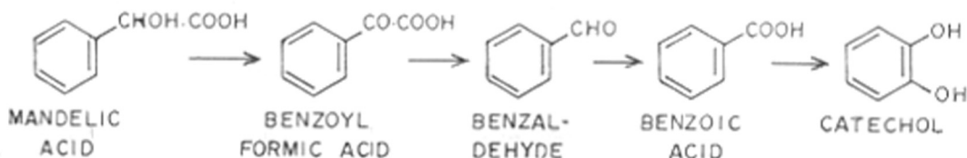
FIG. VI METABOLISM OF MANDELIC ACID
