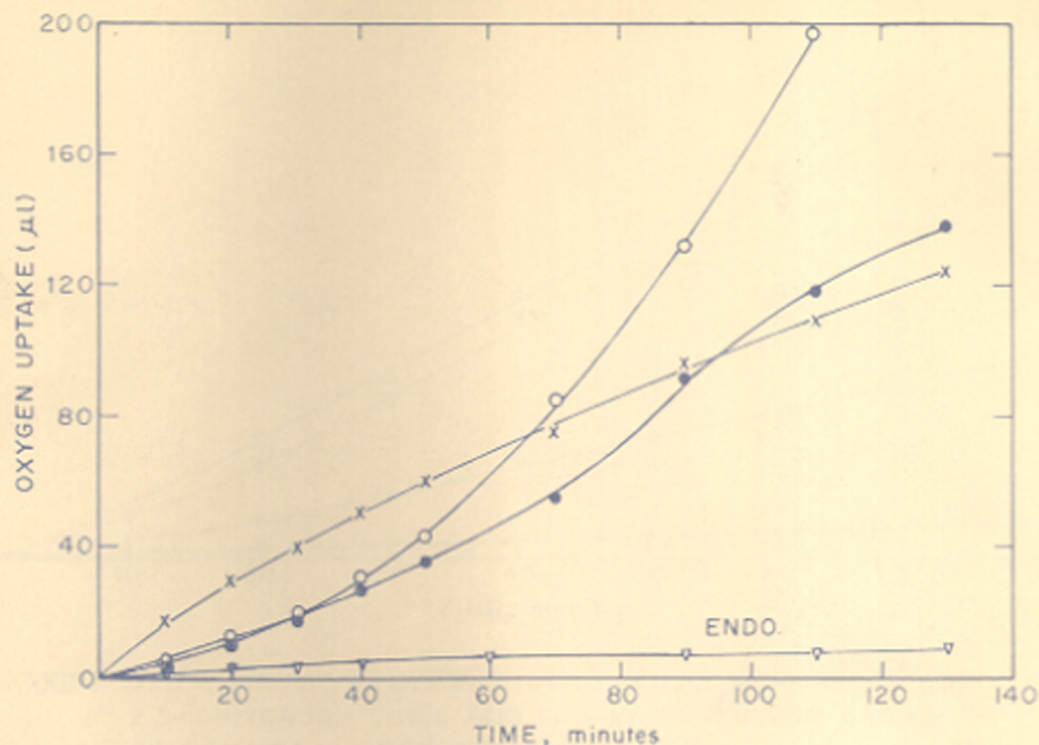
FIG. XXXI a. OXIDATION OF 2,3-DIHYDROXY CUMIC ACID (x—x) CUMIC ACID (o—o) AND P-CYME (•—•) BY 2,3-DIHYDROXY CUMIC ACID GROWN CELLS. (1.46 mg. DRY WEIGHT / FLASK).
