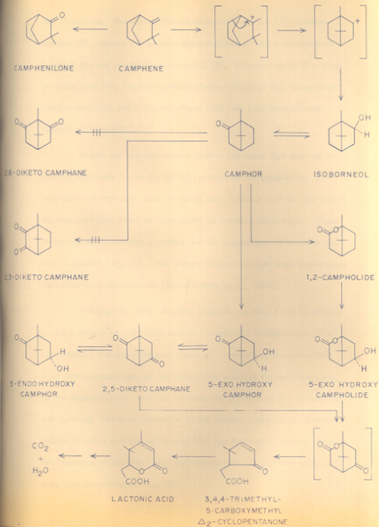
FIG. VII. PROBABLE PATHWAY FOR THE DEGRADATION OF CAMPHENE
