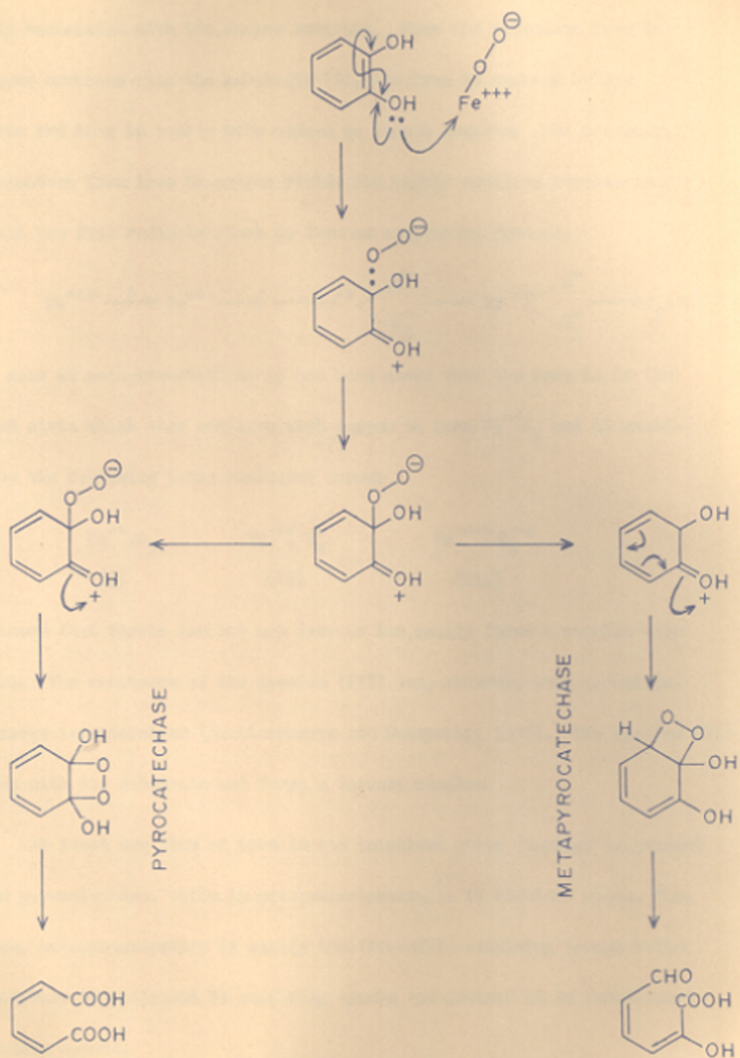
FIG. XXXVII PROPOSED MECHANISM FOR THE REACTION OF METAPYROCATECHASE AND PYROCATECHASE
