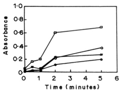
Figure 1.9: Change in relative carbonyl absorption with time. Measured at 1735 cm -1 with CH 2 scissoring peak at 1470 cm -1 as internal standard. LDPE grafted with GA and GMA with acetone as solvent
