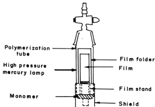
Figure 1. 3: Apparatus of vapor phase photografting
