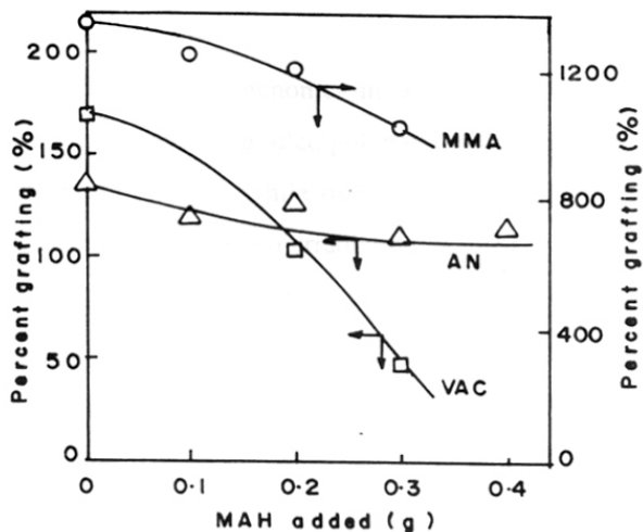
Figure 1.13: Vapor phase photografting on LDPE film sensitized with BPO. Quantity of monomer: 2 mL, Irradiation: 60°C, 60 min, concentration of BPO: 0.3 wt%
