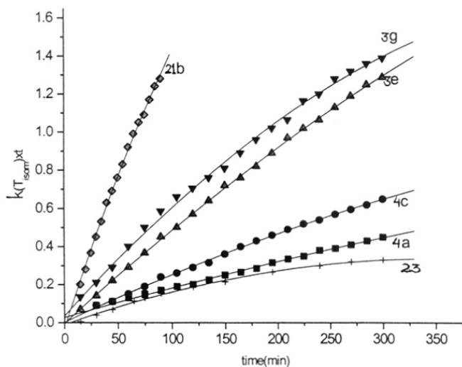
Figure 5.7: Plots of k(T_{\text{isom}})xt vs time( t ) for the semicrystalline and amorphous azo polymer
