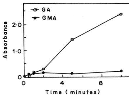
Figure 1.10: Polypropylene grafted with GA and GMA as a function of irradiation time. The relative absorbance of the carbonyl peak at 1740\text{ cm}^{-1} normalized against methylene scissoring at 1470\text{ cm}^{-1} was measured with ATR-IR and transmission IR on 14\text{ }\mu\text{m} thick films
