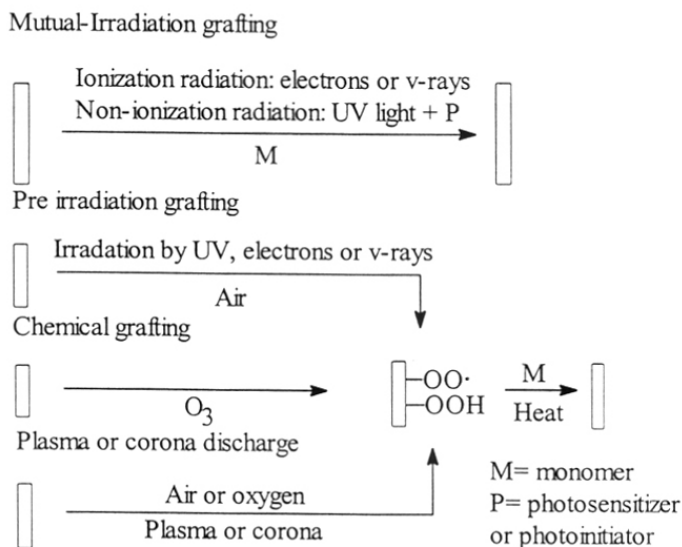
Figure 1.15: Various surface grafting methods
