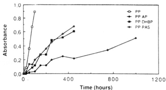
Figure 7.5: Carbonyl absorbance for PP film grafted with hindered amine: 4-amino-2,2,4,4-tetramethylpiperidine (AP), 2,4-dihydroxybenzophenone (DHBP), phenyl 4-aminosalicylate (PAS), irradiated in UVICON at 50°C for different times
