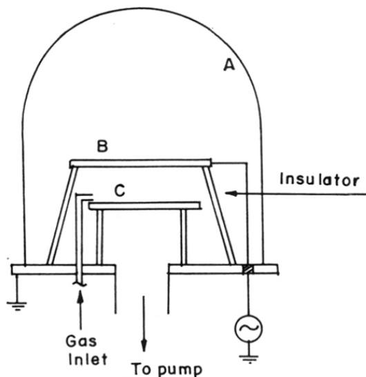
Figure 1.5: Schematic diagram of a bell jar reactor: (A) vacuum chamber (B) rf electrode (C) grounded electrode
