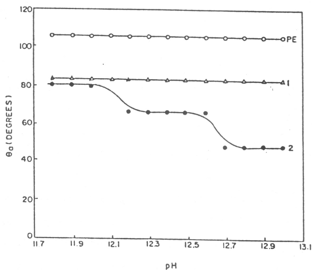
Figure 4.1: Change in contact angle with pH of succinic acid modified poly(ethylene) (o, PE; \Delta , 1; \bullet , 2) (irradiated for 5 h)
