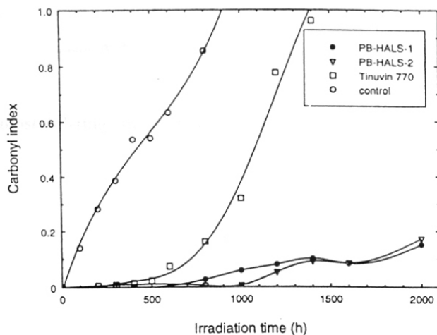
Figure 7.2: Photostabilizing efficiency of polymer-bound HALS and Tinuvin 770 in polyethylene films
