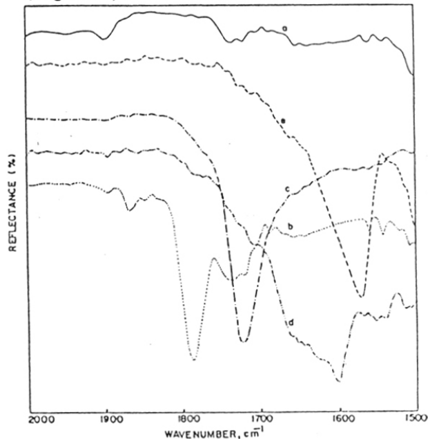
Figure 3.3: ATR-IR spectra of functionalized polyethylene surfaces (a) polyethylene, (b) 1, (c) 2, (d) 3, (e) 4
