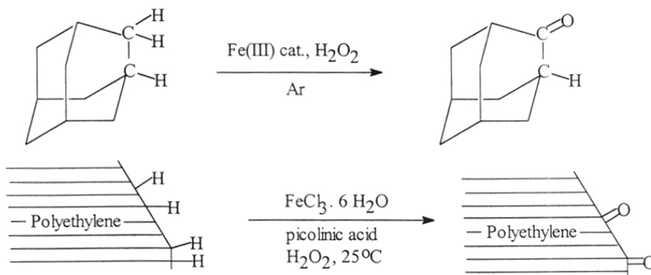
Scheme 1.3: polyolefin oxidation by metal catalyst
