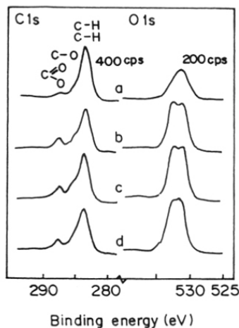
Figure 1.24: XPS spectra of poly(ethylene terephthalate) (a) before cleaning and after cleaning with an ultrasonic cleaner in (b) methanol, (c) acetone and (d) n-heptane
