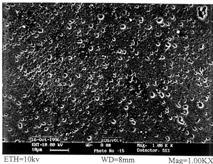
Figure 6.5: SEM microphotographs of sample 4 after plasma exposure
