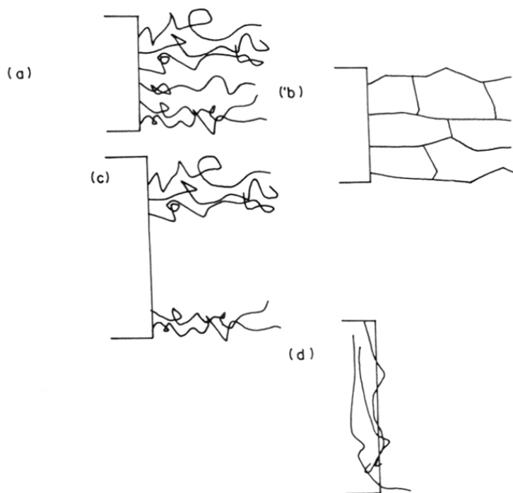
Figure 1.16 (a-d): Possible structure of grafted surfaces: (a) homogeneous coverage of mobile chains, (b) mobile is constrained by cross-linking among grafted chains, (c) non homogeneous coverage, the substrate surface is still exposed, (d) the surface layer contains macromolecular chains both grafted and belonging to the substrate
