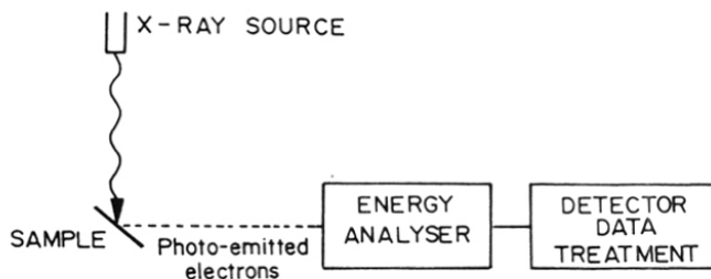
Figure 1.18: Experimental set-up of XPS
