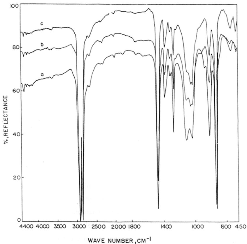
Figure 3.2: ATR-IR spectra of film a: film as such prepared, b: film after exposure to MA, C: film after exposure to UV
