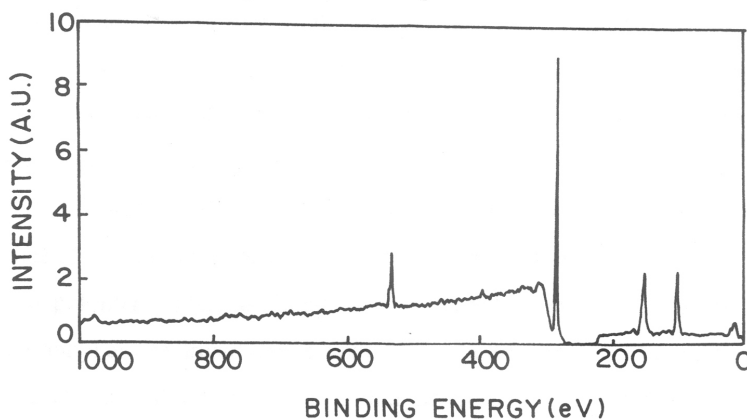
Figure1.20: XPS spectrum of PE contaminated by silicone oil
