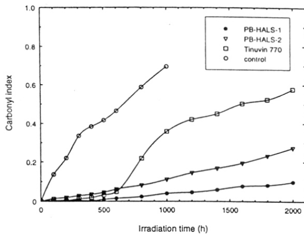
Figure 7.4: Photostabilizing efficiency of polymer-bound HALS and Tinuvin 770 in E-P copolymer films
