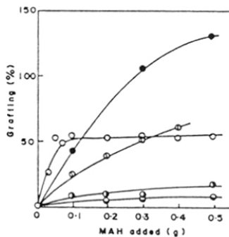
Figure 1.12b: Vapor phase photografting of monomer mixtures of MAH with comonomers on PE film sensitized with BPO. Quantity of monomer, 2 mL; irradiation, 60°C, 60 min. (o) MAH-St; (●) MAH-BMA; (⊖) MAH-EVE (40°C); (⊙) MAH-BVE; (●) MAH-VP
