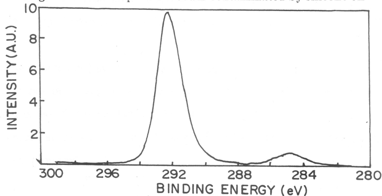
Figure1.21 : Carbon C1s peak of PTFE. The small peak at 285 eV is hydrocarbon contamination
