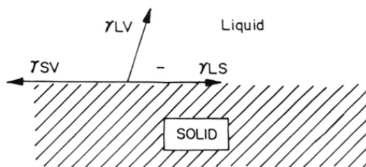
Figure 1.17: The Young equation
