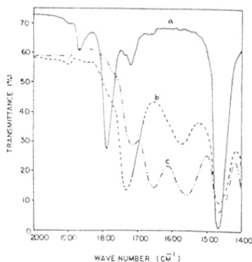
Figure 7.1: FT-IR spectra of polyethylene film. (a) Succinic anhydride modified, (b) PB-HALS-1, (c) PB-HALS-2
