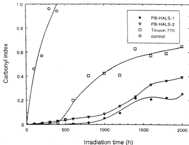
Figure 7.3: Photostabilizing efficiency of polymer-bound HALS and Tinuvin 770 in polypropylene films
