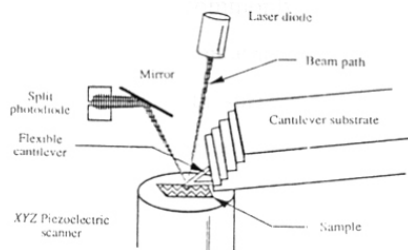
Figure 1.23: An AFM optical sensing system
