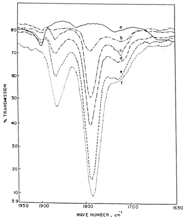
Figure 3.7 Transmission FTIR spectra of modified polyethylene films at various reaction time (a) 0 h, (b) 1 h (c) 2 h (d) 3 h (e) 5 h and (f) 8 h
