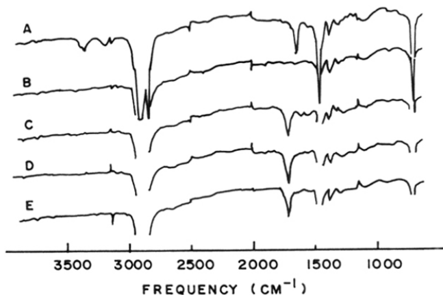
Figure 1.8: ATR-IR spectra of polyethylene film: A, commercial film; B, PE-H, additive free film; C, after oxidation with concentrated chromic acid solution; D, PE-CO 2 H, after treatment with 70% aqueous HNO 3 at 50°C; E, PE-CO 2 H, after extraction with hot 2-propanol
