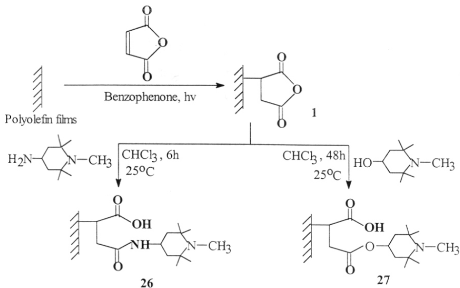
Scheme 7.1: Synthetic route for obtaining polymer-bound hindered amine light stabilizers
