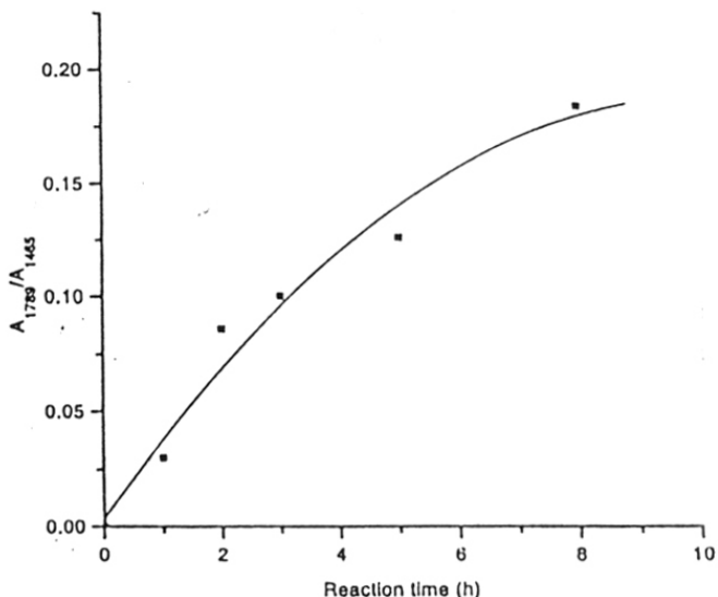
Figure 3.8: Change in the ratio of anhydride: carbon peak area ( area 1789 \text{cm}^{-1} /area 1465 \text{cm}^{-1} ) with reaction time
