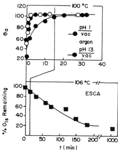
Figure 1.25: Top: The advancing contact angle ( \theta_a ) of water on PE-CO 2 H as a function of the time the polymer had been heated at 100 o C. samples were heated under vacuum or under argon prior to determination of \theta_a with water at either pH 1 or pH 13. The value of \theta_a on PE-H does not change under these conditions. Bottom: The normalized XPS (ESCA) O 1s signal intensity obtained from PE-CO 2 H as a function of time at 106 o C. Samples were heated under argon prior to examination by XPS
