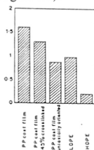
Figure 1.7: Etching rate of polyolefins by chromic acid at 70°C
