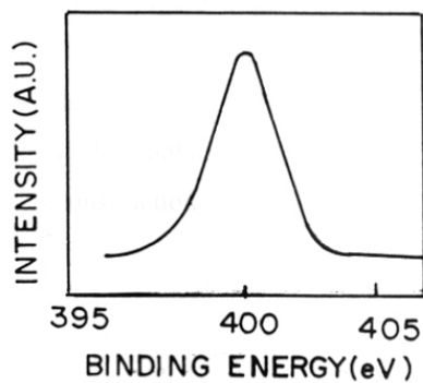
Figure 4.4: XPS spectra of nitrogen of sample 15
