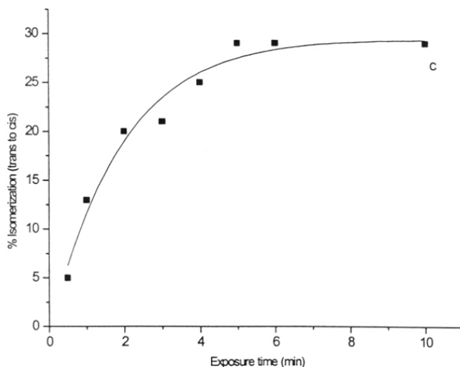
Figure 5.8: Conversion to cis as a function of UV irradiation time at \lambda_{\text{max}}(t) for sample 4a
