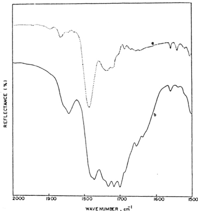
Figure 3.4: ATR-FTIR spectra of film (a) 1 , (b) Commercial sample of melt functionalized maleated polyethylene
