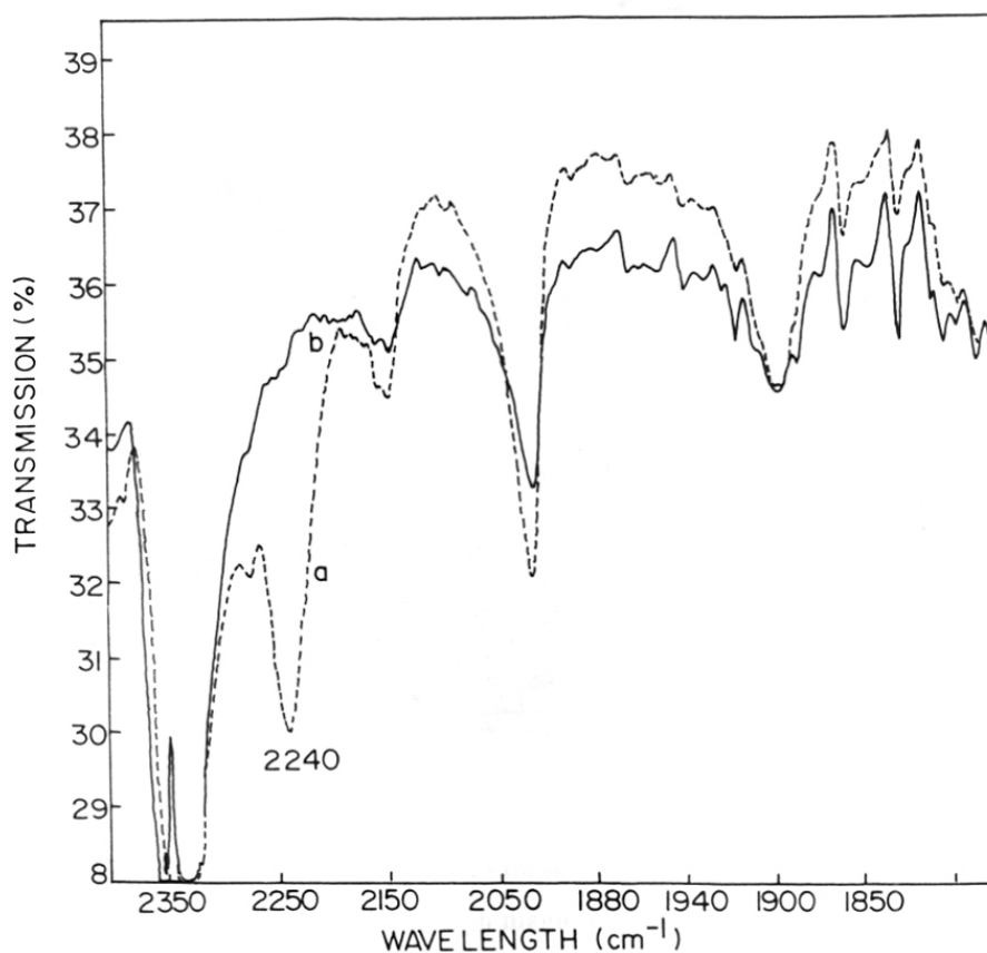
Figure 6.6: FTIR spectra of sample 25 : (a) before heating (b) after heating
