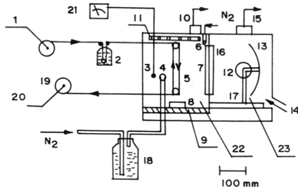
Figure 1.4: Sketch of continuous surface photografting system (1) film feed roll, (2) presoaking solution, (3) thermocouple (screened from UV lamp), (4) vapor inlet of monomer and initiator, (5) running rolls, (6) nitrogen inlet, (7) quartz window, (8) container of solid monomer, (9) electric heater, (10) exhaust outlet, (11) cooling water pipe, (12) UV lamp, (13) parabolic reflector, (14) air inlet, (15) air outlet, (16) screen, (17) lamp support, (18) monomer and initiator bubble solution, (19) take-off roll, (20) driving motor, (21) temperature indicator, (22) reaction chamber, and (23) lamp box
