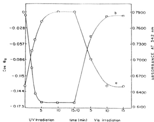
Figure 5.5: Photoinduced changes in absorbance (a) and wettability (b) (sample 4a)
