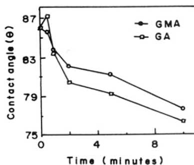
Figure 1.11: Advancing contact angle measurements of water against LDPE grafted with GA and GMA at different UV irradiation times. Acetone was used as solvent
