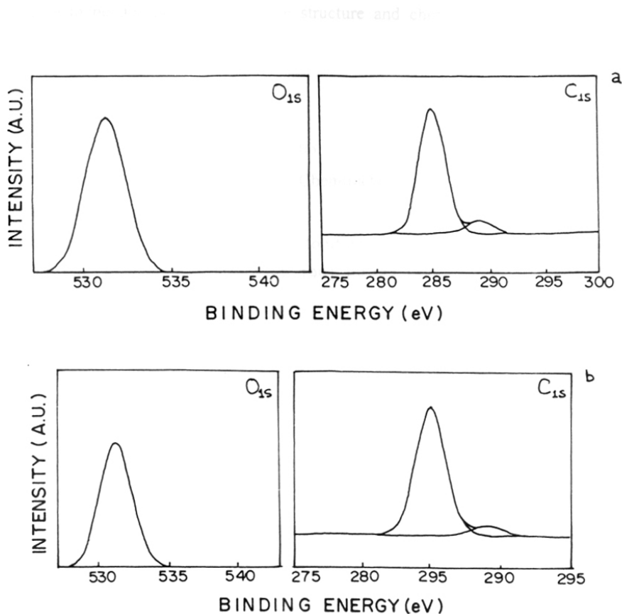
Figure 4.5: XPS spectra of sample 2, a: before heating, b: after heating
