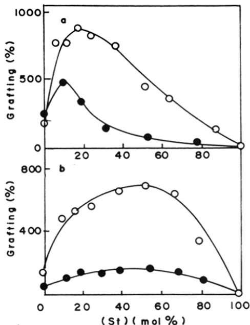
Figure 1.12a: Vapor phase photografting of monomer mixtures of St with AN, GMA, AA and MAA on PE film sensitized with BPO: (a) (O) St-AN; (●) St-GMA; (b) (O) St-AA, (●) St-MAA. Quantity of monomer, 2 mL; irradiation, 60°C, 60 min
